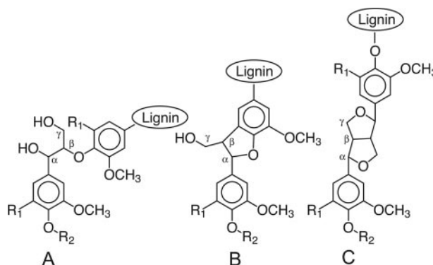
FIG. 1. Principal structures of natural lignins and DHPs. (A) Aryl-glycerol- \beta -aryl ether structures. (B) Phenylcoumaran structures. (C) Resinol structures. R 1 is H for guaiacyl structures and OCH 3 for syringyl structures. R 2 is H for phenolic structures, CH 3 for permethylated phenolic structures, and lignin for nonphenolic structures.
