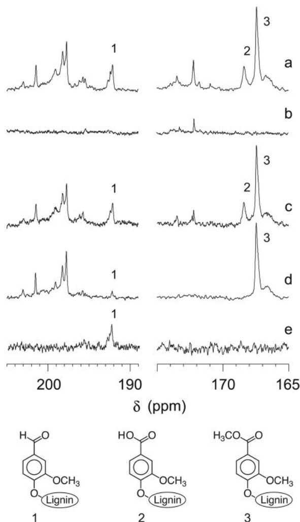
FIG. 3. ^{13}\text{C} NMR results showing (a) a spectrum of the extract from wood decayed by D. concentrica in the presence of permethylated guaiacyl [ \alpha - ^{13}\text{C} ]DHP, (b) a spectrum of the extract from decayed wood that received no DHP, (c) the difference between spectra a and b, (d) a spectrum of undegraded, permethylated, guaiacyl [ \alpha - ^{13}\text{C} ]DHP, and (e) a DEPT spectrum of the extract from wood decayed in the presence of permethylated guaiacyl [ \alpha - ^{13}\text{C} ]DHP. Spectra a and b were normalized with respect to the amount of wood lignin present by equalizing the signal from C-2/C-6 in syringyl aromatic carbons (guaiacyl DHP does not contribute in this region). Spectra a and d were normalized with respect to the amount of DHP present by equalizing the signal from \text{C}_\alpha in resinol structures (this carbon was present at a very low abundance in the wood lignin). The samples were dissolved in 400 \mu\text{l} of acetone- \text{d}_6 - \text{D}_2\text{O} (4:1), and the spectra were obtained with a Bruker DPX 250-MHz spectrometer (62.9 MHz for ^{13}\text{C} ). The qualitative experiments shown in spectra a to d were acquired with a standard power-gated sequence, a 0.5-s delay, and 150,000 scans. Quantitative experiments (not shown) were performed with an inverse-gated sequence, a 15-s delay, a 90^\circ pulse, and 25,000 scans. For spectrum e, the standard Bruker DEPT135 sequence was run for 30,000 scans. In all cases, the acetone signal at 29.8 ppm was used as the internal reference. Structures corresponding to signal assignments 1 to 3 are shown below the spectra. The assignments were confirmed by measuring carbonyl chemical shifts ( \delta ) for 3,4-dimethoxybenzaldehyde, 3,4-dimethoxybenzoic acid, and 3,4-dimethoxybenzoate methyl ester. The new signals at 172 to 174 ppm in spectrum c may represent aliphatic carboxyl groups resulting from \text{C}_\alpha -aryl cleavage of the DHP (1).
