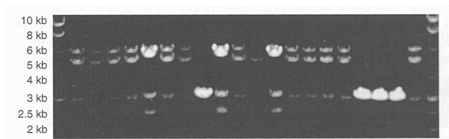
Fig. 3. Restriction digestion of the four piece ligation clones. About 0.5 \mu g of plasmid DNA were digested by 20 U SfiI enzyme for 1 h in a total volume of 20 \mu L, and 5 \mu L samples were loaded onto a 0.8% agarose gel. The first and last lane were loaded with 0.2 \mu g of 1 kb DNA ladder (Promega). The rest of the lanes were loaded with SfiI digested four piece ligation products.
