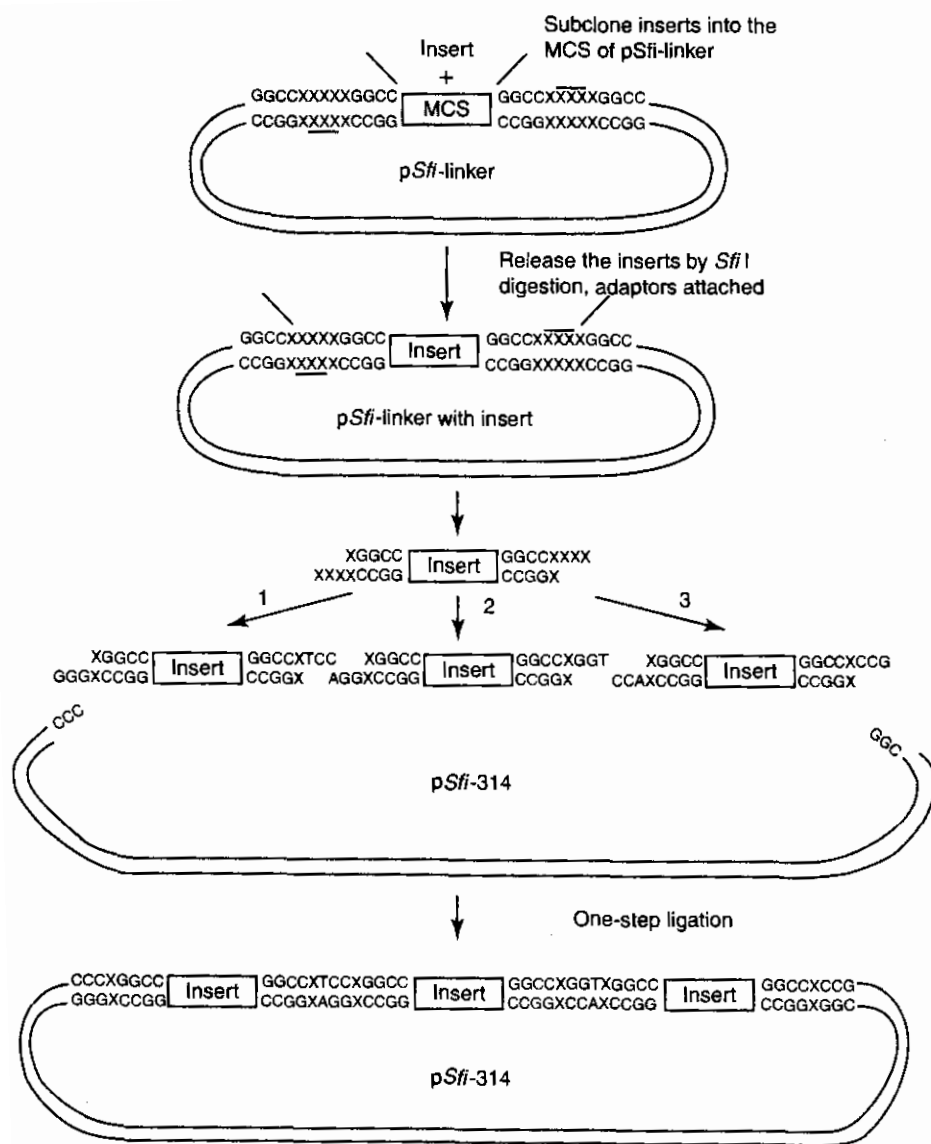
Fig. 1. Experimental strategy for PCR free Sfi I assembly method. In the first step, desired inserts were subcloned to the pSfi-linker vector through Apa I and Bam HI. In the second step, inserts were released from the linker vector by Sfi I digestion, three base adaptors were attached to 5' ends of the insertion on digestion. Finally inserts were joined together through these compatible adaptors.
