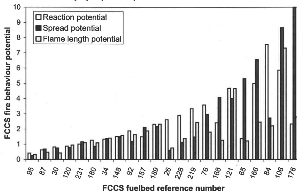
Fig. 2. Fuel Characteristic Classification System (FCCS) reaction potential, spread potential, and flame length potential for randomly selected FCCS fuelbeds, sorted from the lowest to highest surface fire behaviour potential. The component potentials range from 0 to 10, scaled such that the highest rated fuelbed from the family of 216 fuelbeds received a value of 10. FCCS fuelbed 26, interior ponderosa pine – limber pine forest; fuelbed 30, turbinella oak – mountain mahogany shrubland; fuelbed 34, Douglas-fir – interior ponderosa pine – Gambel oak forest; fuelbed 65, purple tussockgrass – California oatgrass grassland; fuelbed 76, slash pine – molassas grass forest; fuelbed 84, Ohio – Broomsedge bluestem savanna; fuelbed 87, black spruce – feathermoss forest; fuelbed 92, aspen – paper birch – white spruce – black spruce; fuelbed 95, willow – alder shrubland; fuelbed 106, red spruce – balsam fir forest; fuelbed 120, oak – pine – mountain laurel forest; fuelbed 121, oak – pine – mountain laurel forest; fuelbed 148, jack pine forest; fuelbed 157, loblolly pine – shortleaf pine – mixed hardwoods forest; fuelbed 166, longleaf pine – three-awned grass – pitcher plant savanna; fuelbed 168, little gallberry – fetterbush shrubland; fuelbed 176, smooth cordgrass – black needlerush grassland; fuelbed 180, red maple – oak – hickory – sweetgum forest; fuelbed 189, sand pine – oak forest; fuelbed 219, ponderosa pine – white fir – trembling aspen forest; fuelbed 228, interior ponderosa pine – limber pine forest; and fuelbed 231, Gambel oak – juniper – ponderosa pine forest.
