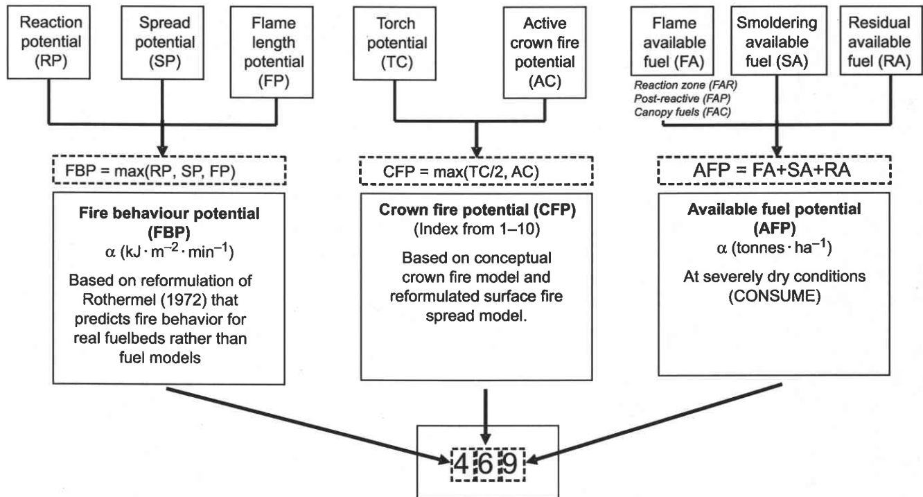
Fig. 1. Fuel Characteristic Classification System (FCCS) fire potentials are expressed as a three-digit number representing the intrinsic capacity of a fuelbed to produce fire behaviour and fire effects that may be parsed into as many as 12 components. There are three categories of FCCS fire potentials (surface fire behavior potential (FBP), crown fire potential (CFP), and available fuel potential (AFP)), each of which combine component FCCS fire potentials (e.g., FBP combines reaction potential (RP), spread potential (SP), and flame length potential (FP)).
