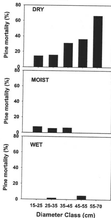
Fig. 3. Diameter distributions of overstory trees (DBH > 15 cm) killed following experimental prescribed fires in long-unburned longleaf pine forests in northern Florida, USA. No overstory pines died in the no-burn control treatment.
