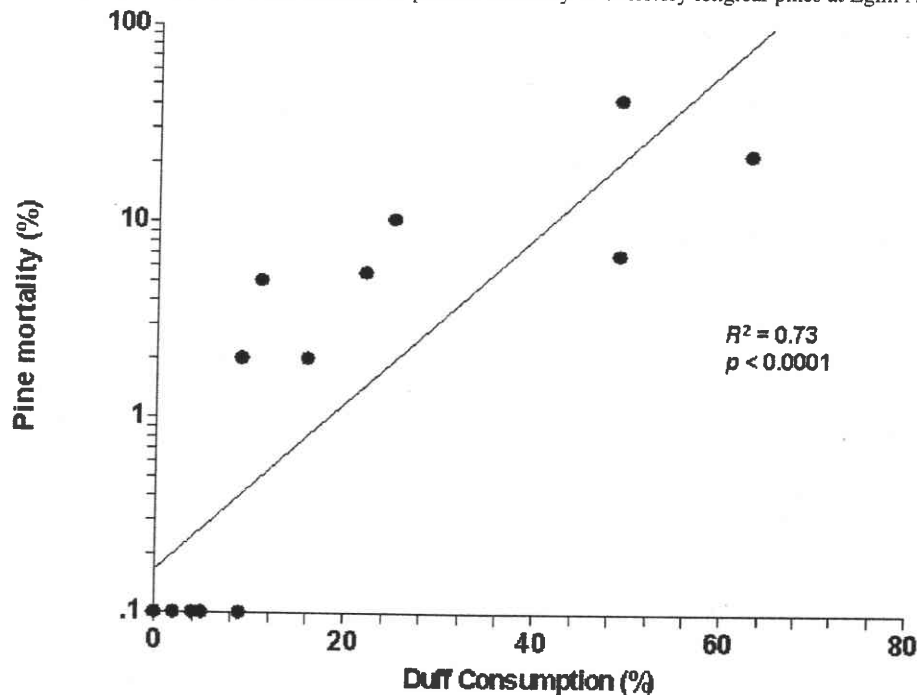
Fig. 4. Relationship between duff consumption and cumulative postfire mortality of overstory longleaf pines at Eglin Air Force Base, Florida.
