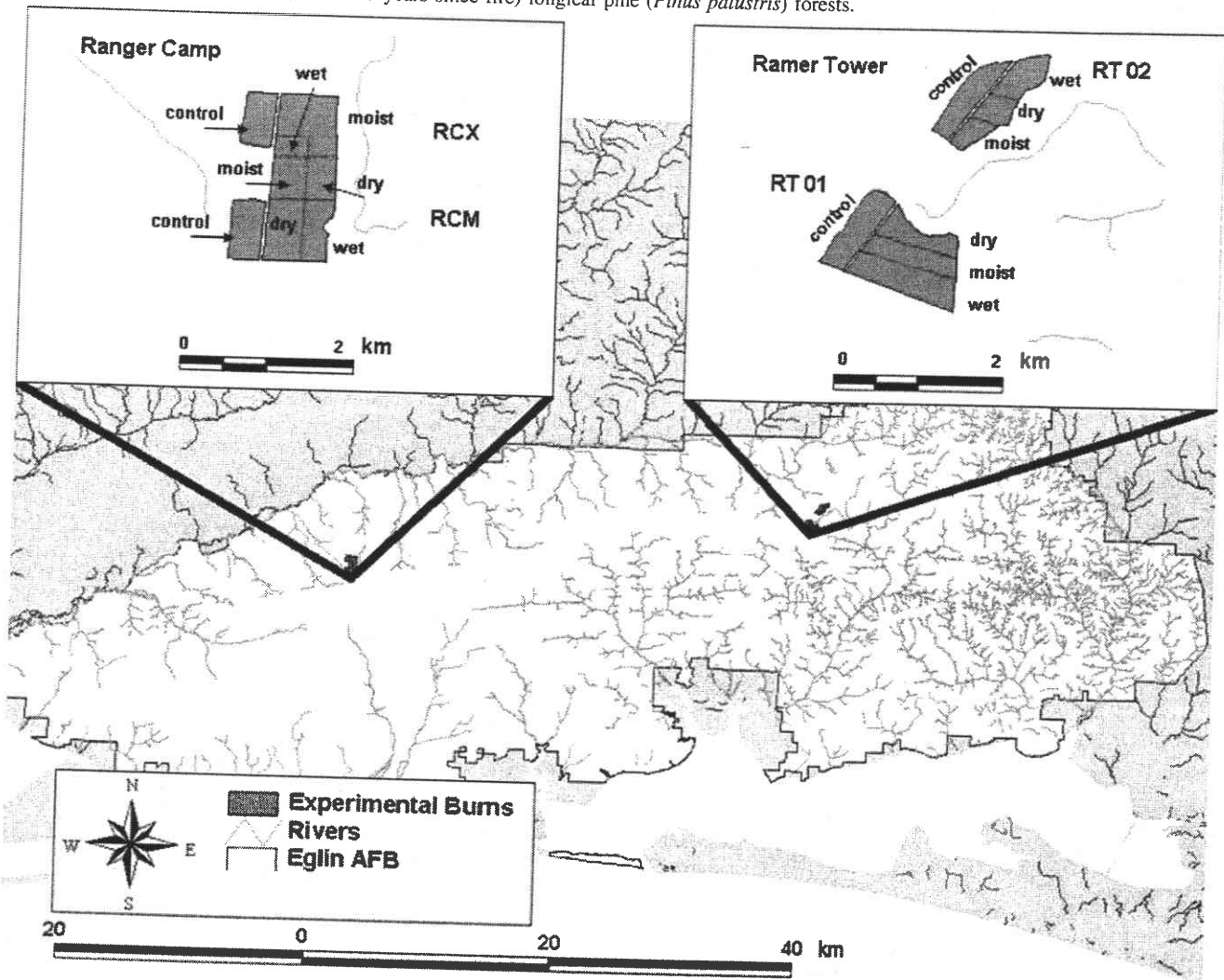
Fig. 1. Study site locations in northern Florida of experimental prescribed fires to examine correlates of mortality resulting from reintroduction of fire into fire-excluded (ca. 35–45 years since fire) longleaf pine ( Pinus palustris ) forests.
