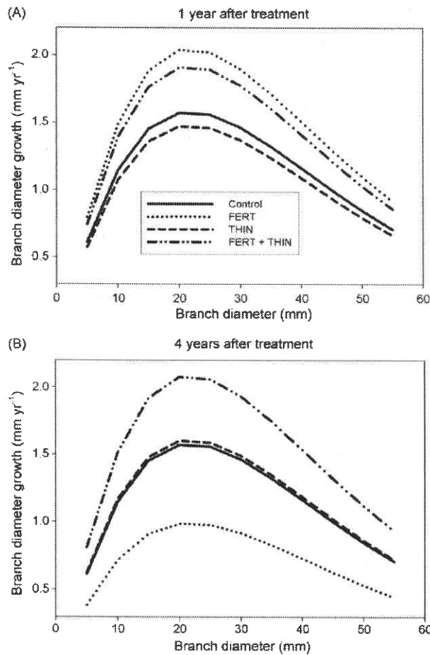
Fig. 3. Predicted branch diameter growth ( \text{mm year}^{-1} ) for a mid-crown whorl branch over initial branch diameter (mm) one (graph A) and four (graph B) years following treatment.
