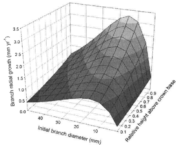
Fig. 4. Predicted branch radial growth using equation (1) over initial branch diameter (mm) and relative height above crown base. The other covariates were set at their mean levels, which were 5 \text{ cm}^2 , 50 \text{ cm}^2 , and 10 \text{ m} for crown sparseness, tree basal area growth, and height to crown midpoint, respectively.
