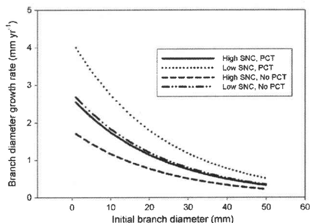
Fig. 2. Predicted branch diameter growth (mm year -1 ) for a mid-crown whorl branch over initial branch diameter (mm) at varying levels of Swiss needle cast (SNC) disease with and without precommercial thinning (PCT). The difference levels of SNC are high (foliage retention = 1.5 years) and low (foliage retention = 3.5 years).
