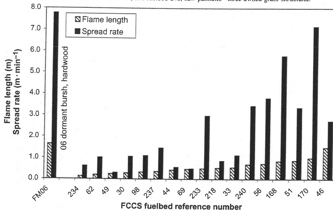
Fig. 9. A sample of Fuel Characteristic Classification System (FCCS) fuelbeds with predicted spread rates and flame lengths similar to fuel model 6 (dormant brush) at fuel moisture scenario D2L2 and at 1.79 \text{ m}\cdot\text{s}^{-1} midflame wind speed. FCCS fuelbed 30, turbinella oak–mountain mahogany shrubland; fuelbed 33, Gambel oak–sagebrush shrubland; fuelbed 44, scrub oak–chaparral shrubland; fuelbed 46, chamise chaparral shrubland; fuelbed 49, creosote bush shrubland; fuelbed 51, Coast sage shrubland; fuelbed 56, sagebrush shrubland; fuelbed 62, Vaccinium –heather shrublands; fuelbed 69, western juniper–sagebrush–bitterbrush shrubland; fuelbed 98, marsh Labrador tea–lingonberry tundra shrubland; fuelbed 168, little gallberry–fetterbush shrubland; fuelbed 170, pond pine–little gallberry–fetterbush shrubland; fuelbed 218, Gambel oak–sagebrush shrubland; fuelbed 233, sagebrush shrubland; fuelbed 234, sagebrush shrubland; fuelbed 237, Vaccinium –heather shrublands; and fuelbed 240, saw palmetto–three-awned grass shrubland.
