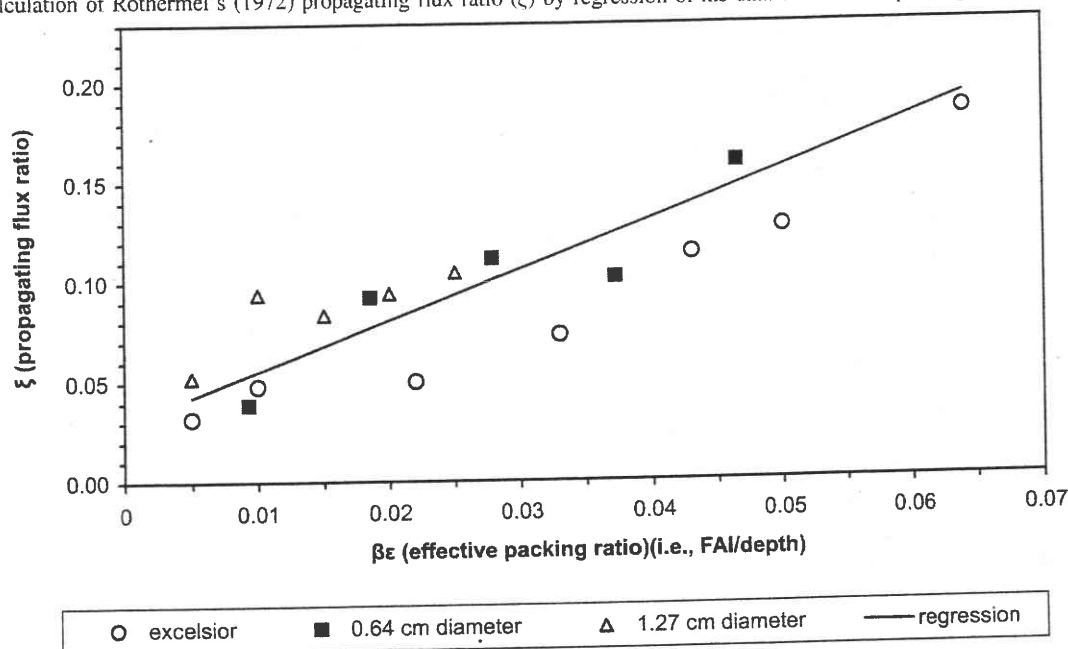
Fig. 1. Recalculation of Rothermel's (1972) propagating flux ratio ( \xi ) by regression of his data on effective packing ratio ( \beta\epsilon ).
