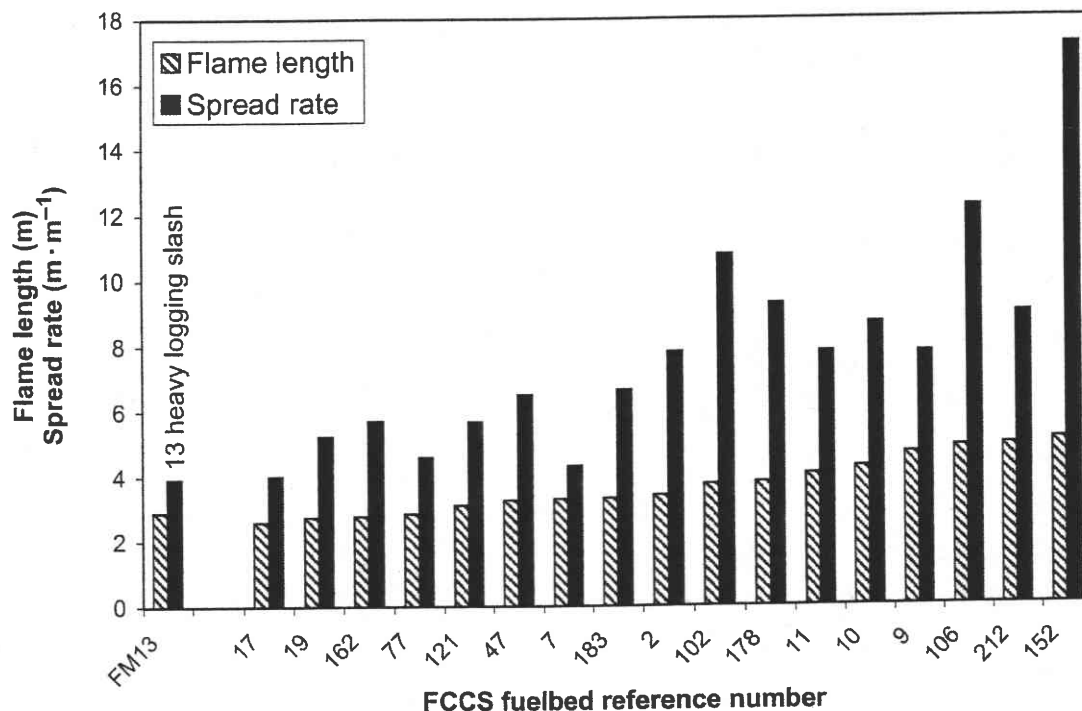
Fig. 12. A sample of Fuel Characteristic Classification System (FCCS) fuelbeds with predicted spread rates and flame lengths similar to fuel model 13 (heavy logging slash) at fuel moisture scenario D2L2 and at 1.79 \text{ m}\cdot\text{s}^{-1} midflame wind speed. FCCS fuelbed 2, western hemlock–western redcedar–Douglas-fir forest; fuelbed 7, Douglas-fir–sugar pine–tanoak forest; fuelbed 9, Douglas-fir–western hemlock–western redcedar–vine maple forest; fuelbed 10, western hemlock–Douglas-fir–Sitka spruce forest; fuelbed 11, Douglas-fir–western hemlock–Sitka spruce forest; fuelbed 17, red fir forest; fuelbed 19, white fir–giant sequoia–sugar pine forest; fuelbed 47, redwood–tanoak forest; fuelbed 77, eucalyptus plantation forest; fuelbed 102, white spruce forest; fuelbed 106, red spruce–balsam fir forest; fuelbed 121, oak–pine–mountain laurel forest; fuelbed 152, red pine–white pine forest; fuelbed 162, loblolly pine–slash pine forest; fuelbed 178, loblolly pine–shortleaf pine forest; fuelbed 183, loblolly pine–shortleaf pine forest; and fuelbed 212, Pacific ponderosa pine forest.
