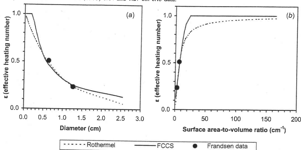
Fig. 2. Comparison of the effective heating number, \varepsilon , derived by Frandsen (1973) with that calculated by the Fuel Characteristic Classification System (FCCS), assuming that a shell of reaction thickness \varsigma_1 = 0.085 cm (or the particle radius, if <0.085 cm) is heated. (a) Comparison between effective heating number and diameter; (b) comparison between effective heating number and surface area-to-volume ratio. Highlighted data points refer to Frandsen's (1973) 0.64 and 1.27 cm crib data.
