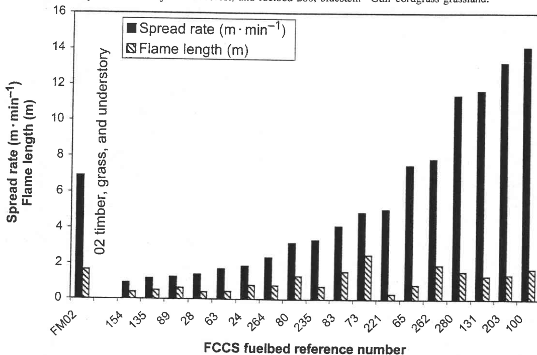
Fig. 7. Sample of Fuel Characteristic Classification System (FCCS) fuelbeds with predicted spread rates and flame lengths similar to fuel model 2 (timber, grass, and understory) at fuel moisture scenario D2L2 (6%–1/2% dead fuel and litter, 30% nonwoody fuel moisture, and 60% shrub fuel moisture), midflame wind speed of 1.79 \text{ m}\cdot\text{s}^{-1} . FCCS fuelbed 24, Pacific ponderosa pine–Douglas-fir forest; fuelbed 28, interior ponderosa pine–limber pine forest; fuelbed 63, showy sedge–alpine black sage grassland; fuelbed 65, purple tussockgrass–California oatgrass grassland; fuelbed 73, koa–pukiawe forest; fuelbed 80, fountain grass grassland; fuelbed 83, molasses grass grassland; fuelbed 89, black spruce–sheathed sedge cottonsedge woodland; fuelbed 100, altai fescue grassland; fuelbed 131, bluestem–Indian grass–switchgrass grassland; fuelbed 135, eastern redcedar–oak–bluestem savanna; fuelbed 154, bur oak savanna; fuelbed 203, sawgrass–Muhlenbergia grassland; fuelbed 221, wheatgrass–ryegrass grassland; fuelbed 235, Idaho fescue–bluebunch wheatgrass grassland; fuelbed 262, molasses grass grassland; fuelbed 264, post oak–blackjack oak forest; and fuelbed 280, bluestem–Gulf cordgrass grassland.
