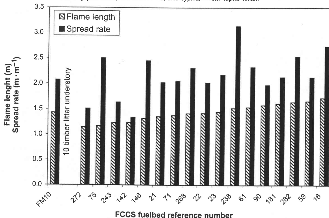
Fig. 11. A sample of Fuel Characteristic Classification System (FCCS) fuelbeds with predicted spread rates and flame lengths similar to fuel model 10 (timber litter understory) at fuel moisture scenario D2L2 and at 1.79 \text{ m}\cdot\text{s}^{-1} midflame wind speed. FCCS fuelbed 16, Jeffery pine–ponderosa pine–Douglas-fir–black oak forest; fuelbed 21, lodgepole pine forest; fuelbed 22, lodgepole pine forest; fuelbed 23, lodgepole pine forest; fuelbed 59, subalpine fir–Engelman spruce–Douglas-fir–lodgepole pine forest; fuelbed 61, whitebark pine–subalpine fir forest; fuelbed 71, Ohio Florida hopbush–kupaoa forest; fuelbed 75, slash pine–New Caledonia pine forest; fuelbed 90, white oak–northern red oak forest; fuelbed 142, trembling aspen–paper birch forest; fuelbed 146, jack pine forest; fuelbed 181, pond pine forest; fuelbed 238, Pacific silver fir–mountain hemlock forest; fuelbed 243, pitch pine–scrub oak shrubland; fuelbed 272, red mangrove–black mangrove forest; fuelbed 282, loblolly pine forest; and fuelbed 288, bald-cypress–water tupelo forest.
