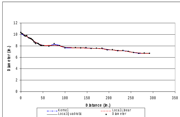
Figure 3. Nonparametric regression fits to one of the southern pine sawlogs.
