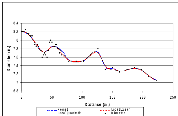
Figure 4. Nonparametric regression fits to one of the southern pine sawlogs.
