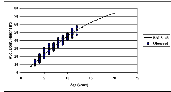
Figure 2. Predicted average dominant and codominant height growth curve implied by equation (4) and observed height measurements.
