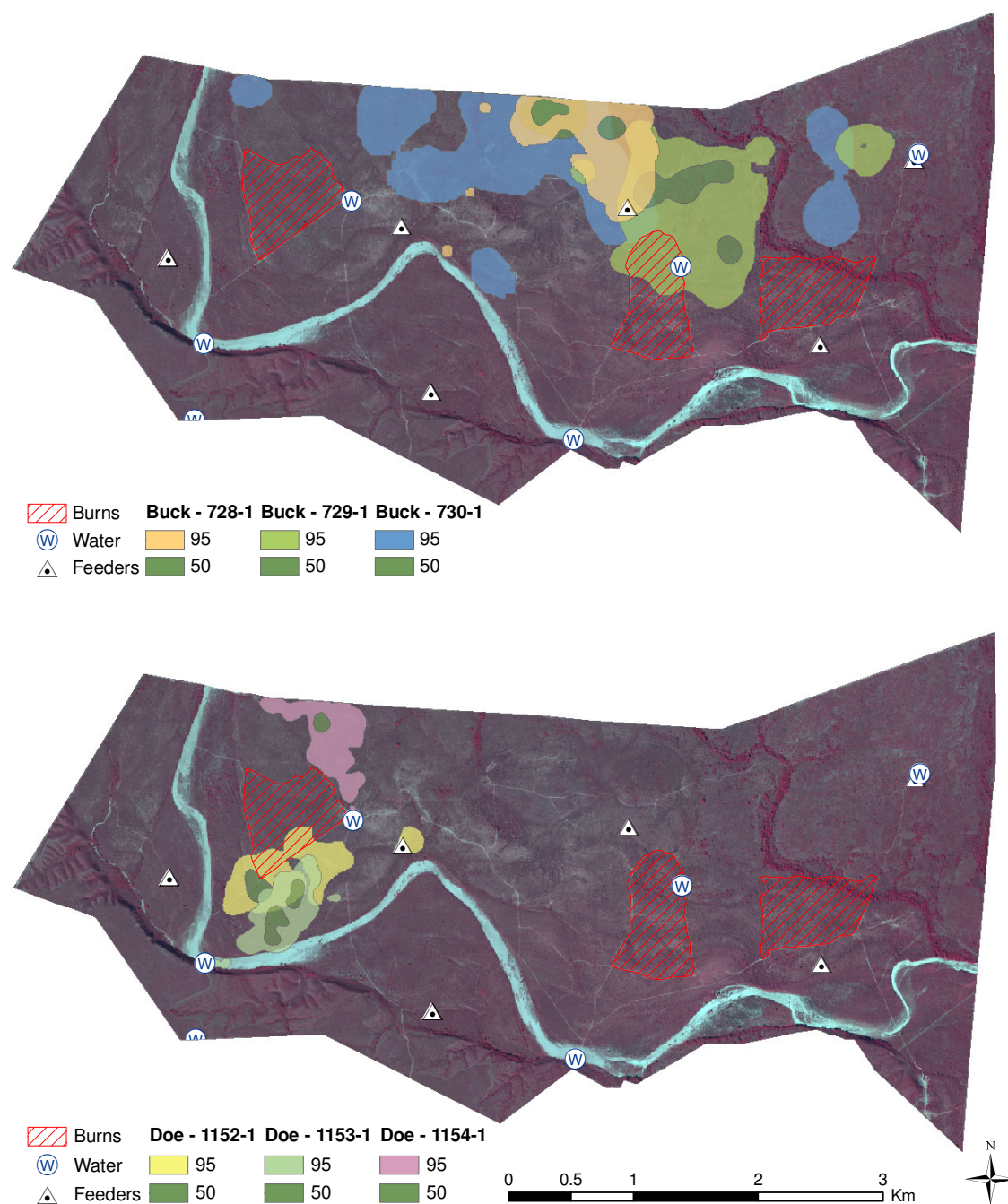
Figure 3. Fixed-kernel density estimates of summer seasonal home ranges of males (top) and females (bottom) in trial 1 (Aug 2005, pre-burn). These distributions are based on hourly fixes collected over 30 days.
