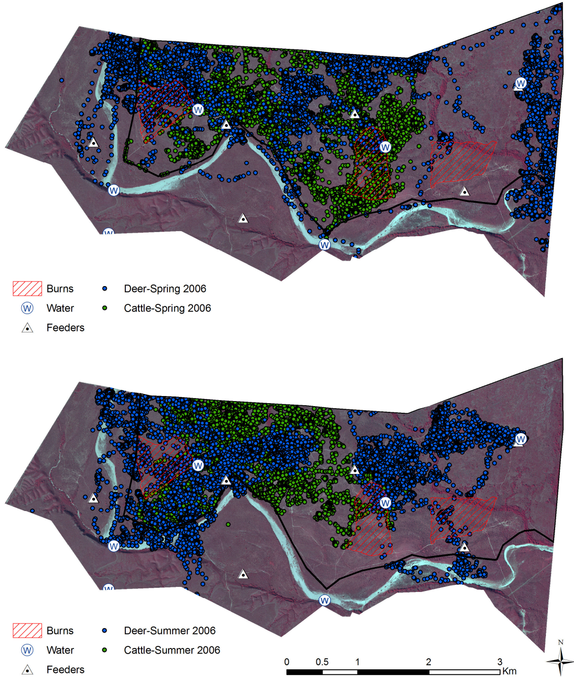
Figure 12. Point distribution of deer (blue) and cattle (green) 5-minute data for 12 days during Spring 2006 (top) and Summer 2006 (bottom).
