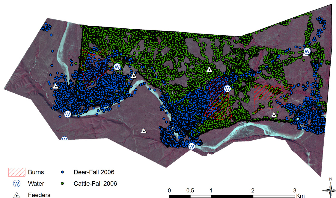
Figure 13. Point distribution of deer (blue) and cattle (green) 5-minute data for 12 days during Fall 2006.
