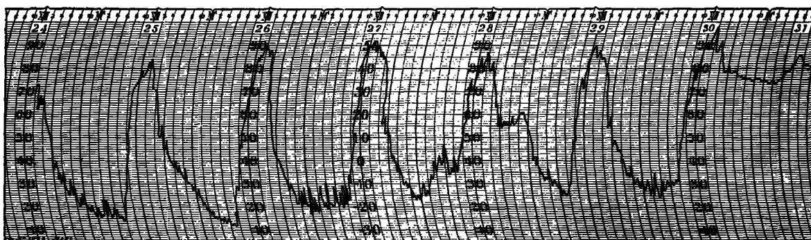
FIG. 2.—Thermogram at Station No. 2 (Park), December 24-31, 1909.
