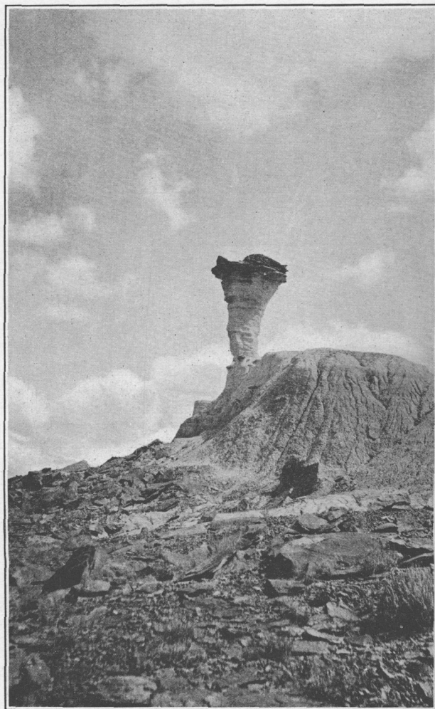
FIG. 1.—Eagle's Nest Rock. The pinnacle shows the height from which the entire region has been eroded by recent water action.
