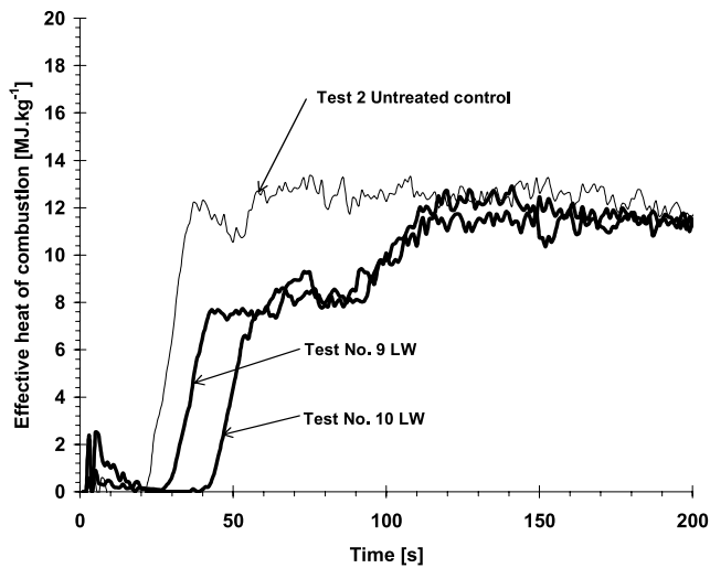
Fig. 5 Effective heat of combustion curves for lime water (LW) specimens (Test nos. 9 and 10) and for one of the untreated control specimens (Test no. 2) for the initial 200 seconds
