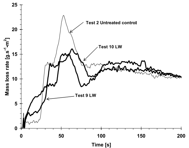
Fig. 6 Mass loss rate curves for lime water (LW) specimens (Test nos. 9 and 10) and for one of the untreated control specimens (Test no. 2) for the initial 200 seconds
