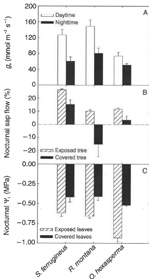
Figure 5. (A) Diurnal and nocturnal mean stomatal conductance ( g_s ), (B) nocturnal sap flow of exposed and covered trees and (C) nocturnal leaf water potential ( \Psi_i ) of exposed and covered leaves of three dominant evergreen cerrado woody species. Bars are means \pm 1 SE of six leaves for \Psi_i , ten leaves for g_s and 4 days of sap flow measurements. Data obtained from Bucci et al. 2004a.
