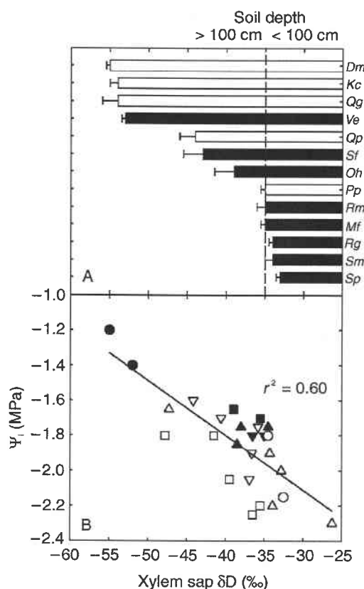
Figure 1. (A) Xylem sap stable hydrogen isotope composition ( \delta D ; \pm SE, n = 3-4 ), near the end of the dry season for eight evergreen (filled bars) and five deciduous (open bars) woody cerrado species. Approximate limit of two distinct soil layers with different water \delta D is indicated by the vertical dashed line. (B) Minimum leaf water potential ( \Psi_l ) in relation to xylem sap \delta D for eight evergreen cerrado species. Each value represents a different individual: Mf, Miconia ferruginata (■); Oh, Ouratea hexasperma (▽); Rg, Myrsine guianensis (△); Rm, Roupala montana (▲); Sm, Schefflera macrocarpa (▼); Sp, Sclerolobium paniculatum (○); Sf, Styrax ferrugineus (□); Ve, Vochysia elliptica (●); Qp, Qualea parviflora ; Pp, Pterodon pubescens ; Qg, Qualea grandiflora ; and Dm, Dalbergia miscolobium . Data are from Jackson et al. (1999) and S.J. Bucci, unpublished data.
