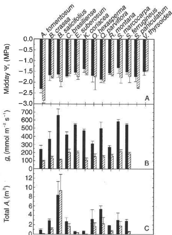
Figure 4. (A) Midday leaf water potentials ( \Psi_l ); (B) mean stomatal conductance ( g_s ); and (C) total leaf area per tree during the wet (filled bars) and dry (lined bars) seasons for the representative cerrado woody species listed in Table 1. Bars are means \pm 1 SE. Measurements were made on three to five leaves per tree (A and B) and two to five trees per species (all panels). Measurements were obtained with a pressure chamber and a steady-state porometer. Data obtained from Bucci et al. 2004a, Bucci et al. 2005 and Scholz 2006.
