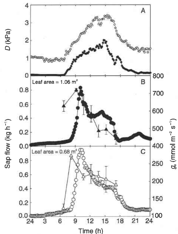
Figure 3. (A) Air saturation deficit ( D ) during typical dry ( \circ ) and wet ( \bullet ) season days. Typical daily courses of sap flow ( \bullet , \circ ) and stomatal conductance ( g_s ; \blacktriangle , \triangle ) during the (B) wet and (C) dry seasons in a dominant evergreen cerrado species ( Schefflera macrocarpa ) at the IBGE research station in central Brazil. Total leaf area per tree during sap flow measurements is shown in each panel. All measurements of sap flow were made by the heat dissipation method (Granier 1985, 1987). Stomatal conductance was measured with a steady-state porometer. Data adapted from Bucci 2001.
