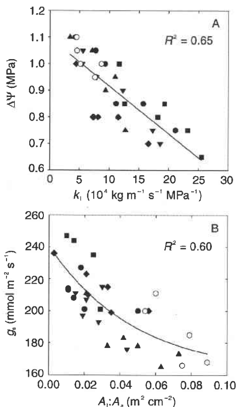
Figure 6. (A) Diurnal variation in leaf water potential ( \Delta\Psi_l ) in relation to leaf specific hydraulic conductivity ( k_l ) and (B) stomatal conductance ( g_s ) in relation to leaf area per unit sapwood area ( A_l:A_s ) for six of the cerrado tree species listed in Table 1. Each value represents one individual of one species: Schefflera macrocarpa (▲); Styrox ferrugineus (●); Kielmeyera coriacea (■); Ouratea hexasperma (▼); Caryocar brasiliense (◆); and Erythroxylum suberosum (○) ( n = 6 for all species). Data obtained from Bucci et al. 2004b.
