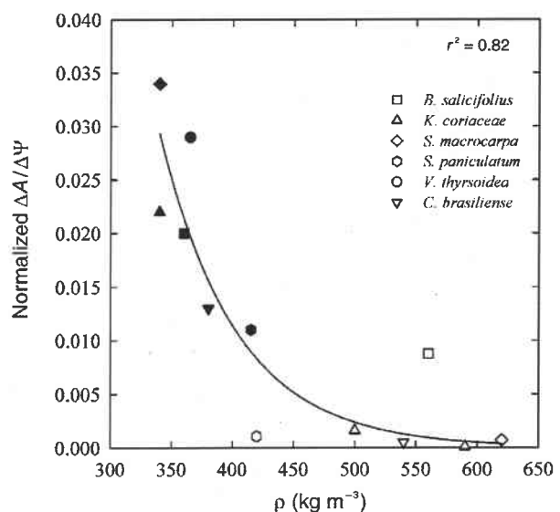
Figure 7. Rate of change in normalized cross-sectional area of sapwood or outer parenchyma per unit change in water potential (Normalized \Delta A / \Delta \Psi ) as a function of sapwood (open symbols) or outer parenchyma (filled symbols) density ( \rho ) for six cerrado tree species. The line is an exponential function fitted to the data ( y = 0.0012 + 11\exp(-0.018x) , P < 0.001 ).
