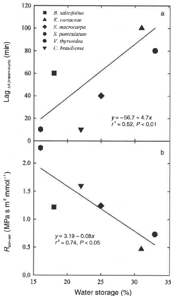
Figure 9. (a) The lag time between the initial morning decline in branch and trunk cross-sectional area and (b) apparent soil-to-leaf hydraulic resistance ( R_{soil-leaf} ) in relation to the relative contribution of internal water storage to total daily water use. The lines are linear regressions fitted to the data.
