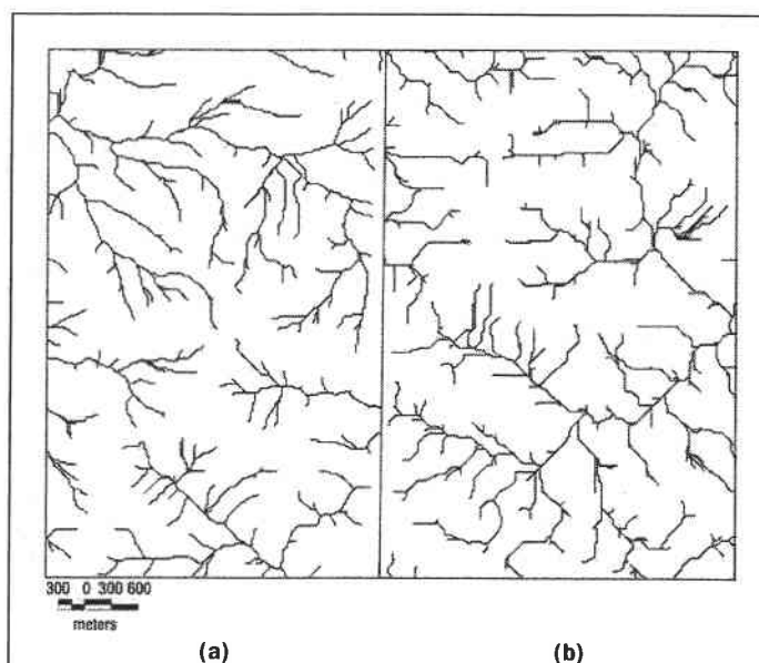
Figure 5. Stream generation comparison between Level 1 and Level 2 30-meter DEMs: (a) Elsie Quadrangle Level 2, 30-meter DEM; (b) Sunset Springs Quadrangle Level 1, 30-meter DEM.
