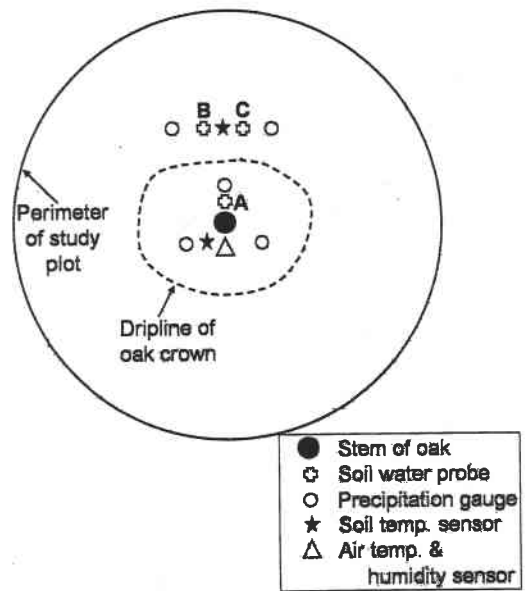
Figure 1 Study plot layout, showing locations of sensors and precipitation gauges in relation to the study tree.
