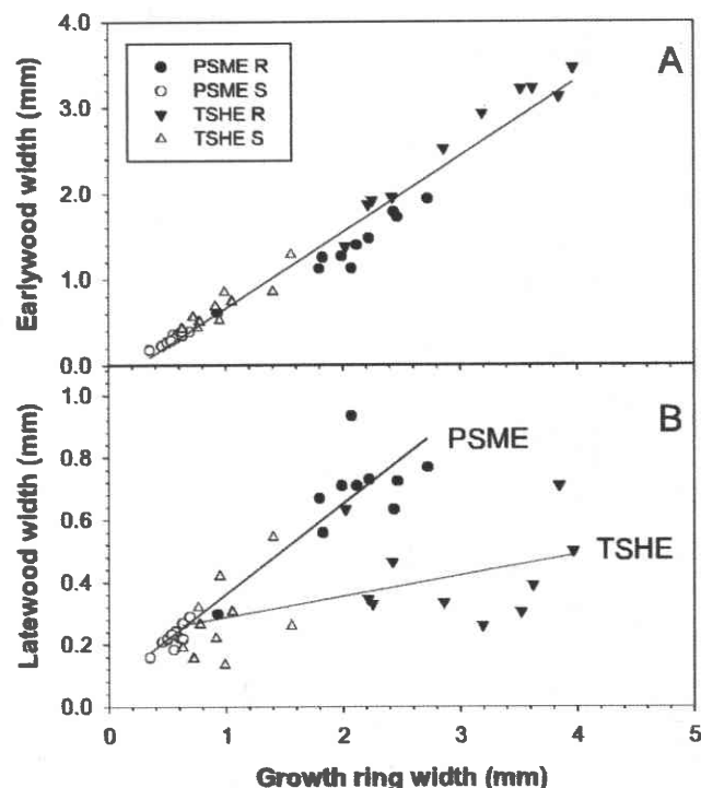
Fig. 2. Relationship between growth ring width and (A) earlywood width ( r^2 = 0.97 , p < 0.0001 ) or (B) latewood width for Douglas-fir ( r^2 = 0.90 , p < 0.0001 ) and western hemlock ( r^2 = 0.26 , p = 0.02 ). See Fig. 1 for abbreviations.
