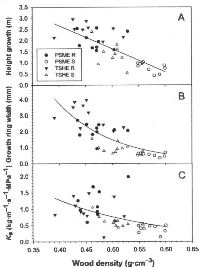
Fig. 5. Relationship between wood density and (A) height growth ( r^2 = 0.59 , p < 0.0001 ), (B) growth ring width ( r^2 = 0.61 , p < 0.0001 ) or (C) specific conductivity ( K_s ) ( r^2 = 0.35 , p = 0.0005 ). See Fig. 1 for abbreviations.
