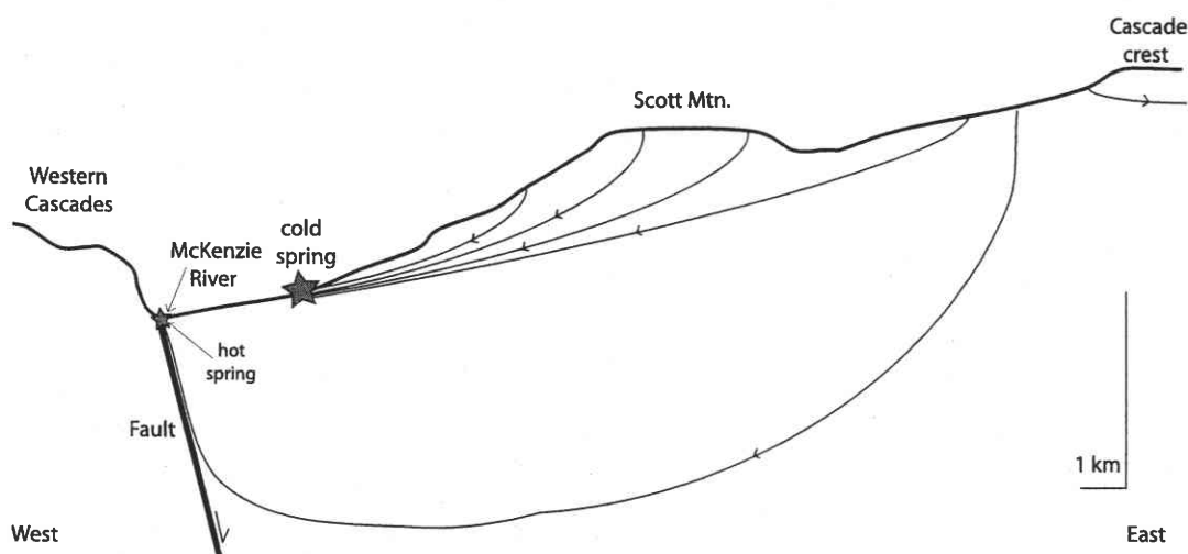
Figure 2. Cross section from the Cascade crest to the Western Cascades along the line in Figure 1b. Actual topography is shown, but flow paths are conceptual. Hot springs occur where deep groundwater flow paths are interrupted by faults [Ingebritsen et al. , 1994], while cold springs are the result of shallower flow paths.
