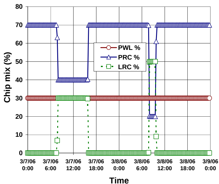
Fig. 3. Time series showing the chip-mix ratios during the residue chip study.
