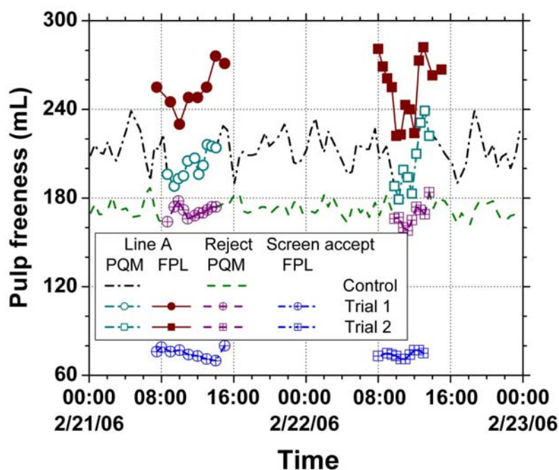
Fig. 4. Time series of pulp freeness measured by Pulp Quality Measurement (PQM) and Lab (FPL) analysis during the whole-log chip study (see Fig. 2).
