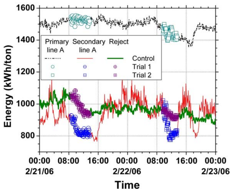
Fig. 9. Time series of specific energy consumption for the primary and secondary refineries for production line A plus the reject refiner during the whole-log chips study.
