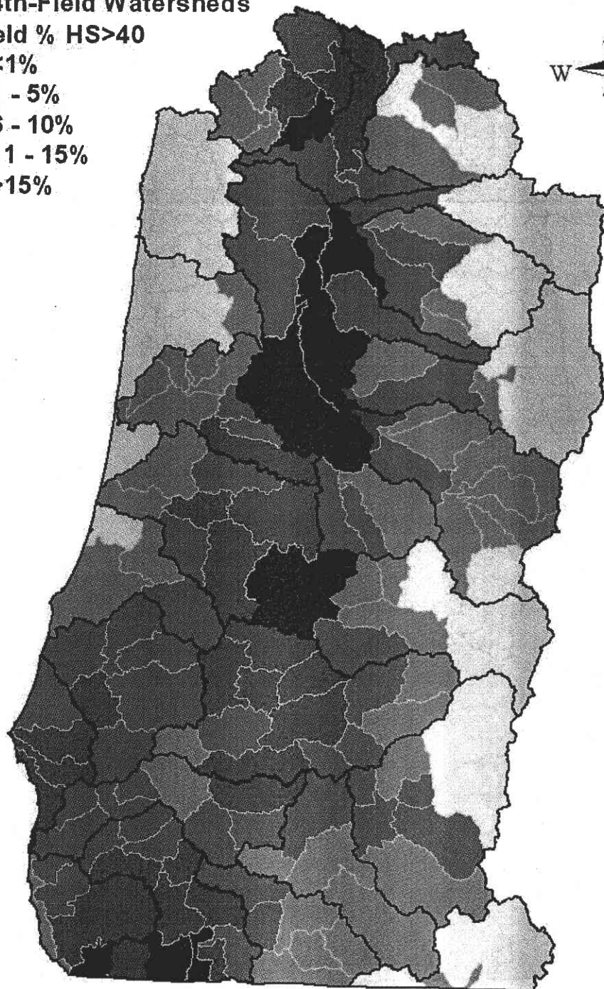
Figure 2-2. A graduated 4 th and 5 th -field watershed map showing the percentage of the watershed's river and stream network that was modeled as suitable habitat (HS>40) for the foothill yellow-legged frog. Percentages ranged from 0-24%. For watersheds that contained suitable habitat, the mean percentage of a watershed's river and stream network that was modeled as suitable was 10%.
