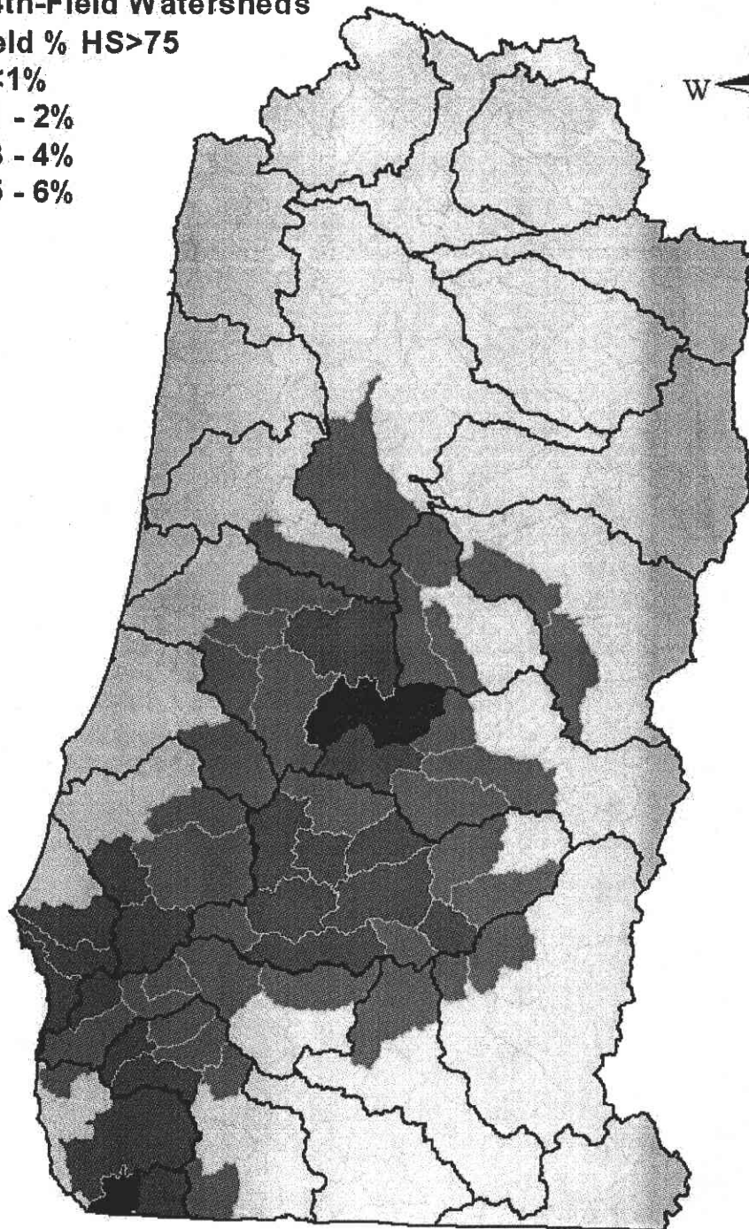
Figure 2-3. A graduated 4 th and 5 th -field watershed map showing the percentage of the watershed's river and stream network that was modeled as optimal habitat (HS>75) for the foothill yellow-legged frog. Percentages ranged from 0-24%. For watersheds that contained suitable habitat, the mean percentage of a watershed's river and stream network that was modeled as optimal was 2%.
