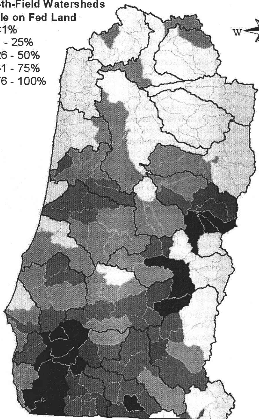
Figure 2-4. A graduated 4 th and 5 th -field watershed map showing the percentage of the watershed's suitable habitat (HS>40) for the foothill yellow-legged frog, that is on Federal Lands (e.g., USFS and BLM). Percentages ranged from 0-100%.
