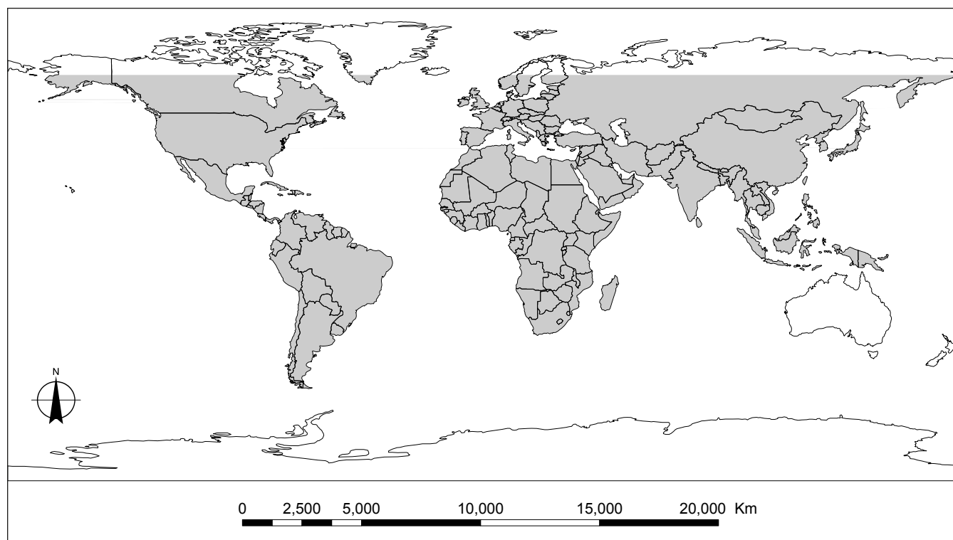
Figure 13—Shuttle Radar Topography Mission (SRTM) coverage (grey area) for 3-arc-second digital elevation models and derived products. Modified from Global Land Cover Facility SRTM figures (Global Land Cover Facility 2005).
