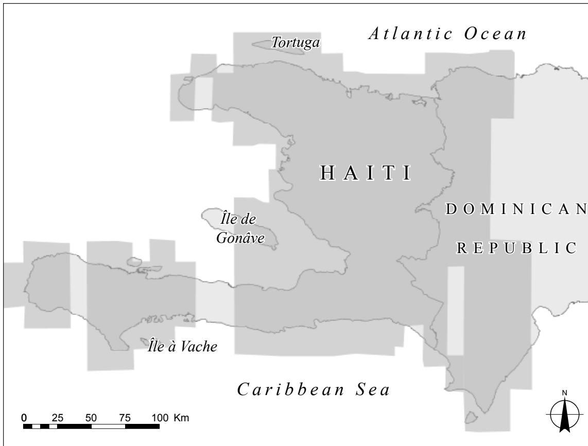
Figure 9—Archived QuickBird satellite images coverage (dark grey area) of Haiti on Digital Globe Image Library. Modified from Digital Globe Image Library search results map (Digital Globe 2005).
