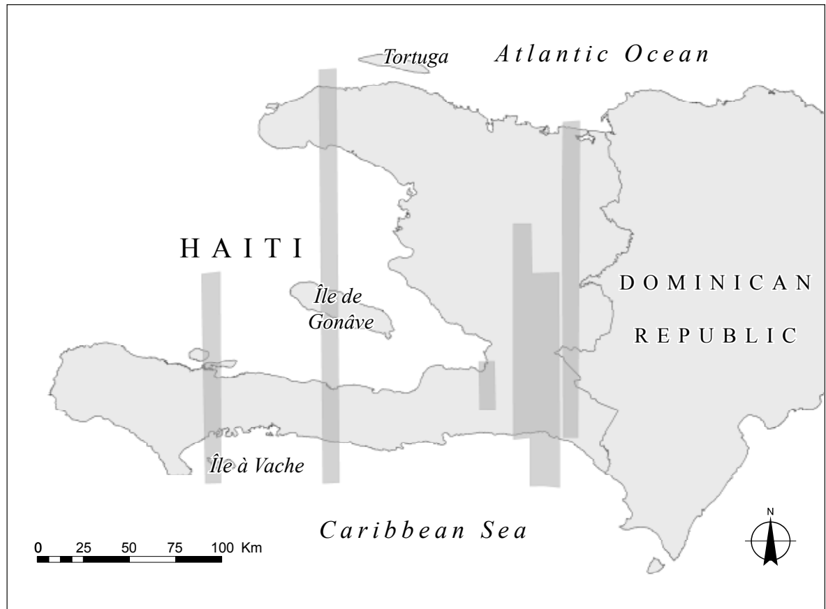
Figure 10—Archived OrbView satellite images coverage (dark grey area) of Haiti on the ORBIMAGE Online Archive Imagery Search Tool. Modified from ORBIMAGE Online Archive Imagery Search Tool search results map (ORBIMAGE 2005).
