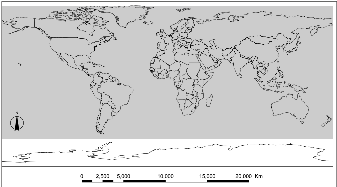
Figure 14—Shuttle Radar Topography Mission (SRTM) coverage (grey area) for 30-arc-second digital elevation models and derived products. Modified from Global Land Cover Facility SRTM figures (Global Land Cover Facility 2005).
