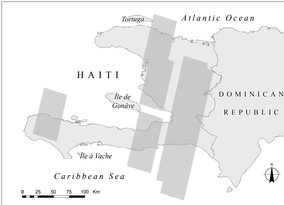
Figure 5—Archived EO-1 ALI satellite image coverage (dark grey area) of Haiti on the USGS Earth Explorer online archive. Modified from the USGS Earth Explorer online archive search results map (U.S. Geological Survey 2005).
