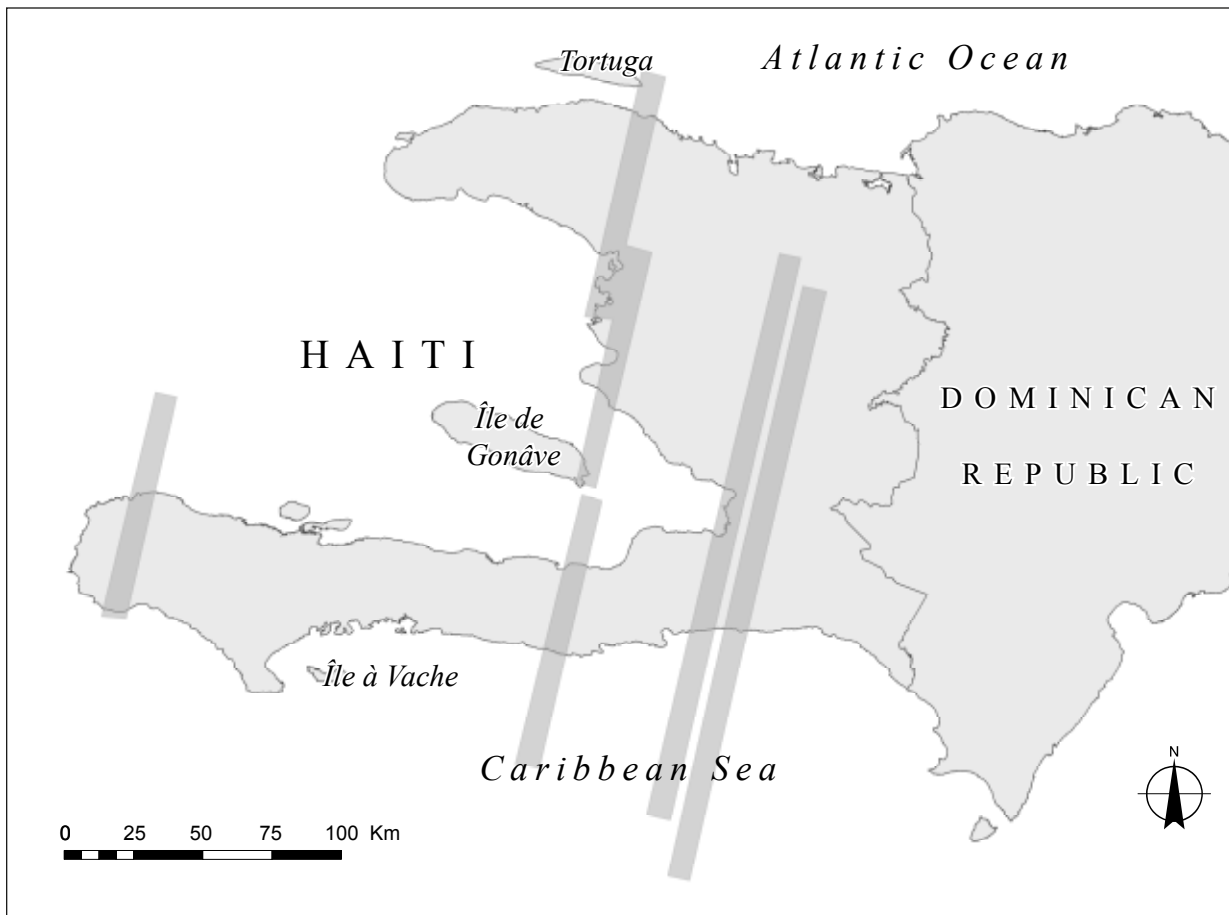
Figure 11—Archived EO-1 Hyperion satellite images coverage (dark grey area) of Haiti on the USGS Earth Explorer online archive. Modified from USGS Earth Explorer online archive search results map (U.S. Geological Survey 2005).
