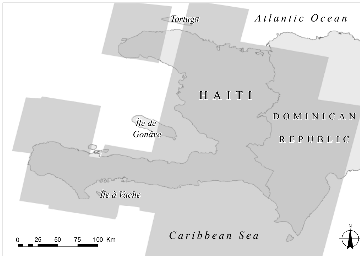
Figure 7—Archived IRS satellite images coverage (dark grey area) of Haiti on CARTERRA. Modified from CARTERRA search results map (Space Imaging 2006).
