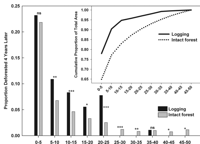
Fig. 3. The proportion of year 2000 logging and intact forest subsequently deforested by 2004 across the Amazon study area at distance classes of 0–50 km from major roads. The Pearson significance of \chi^2 comparisons between the deforestation of logged or intact points per distance class is shown as: ns, nonsignificant; *, P < 0.05 ; **, P < 0.01 ; and ***, P < 0.001 . (Inset) The cumulative distribution of logged forest (1999–2002) and intact forest as a function of distance from main roads.
