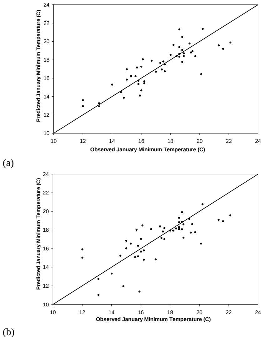
Figure 5. Scatterplots of predicted versus observed mean 1963-95 January minimum temperature for Puerto Rico, Vieques, and Culebra: (a) PRISM; and (b) HYPs.
