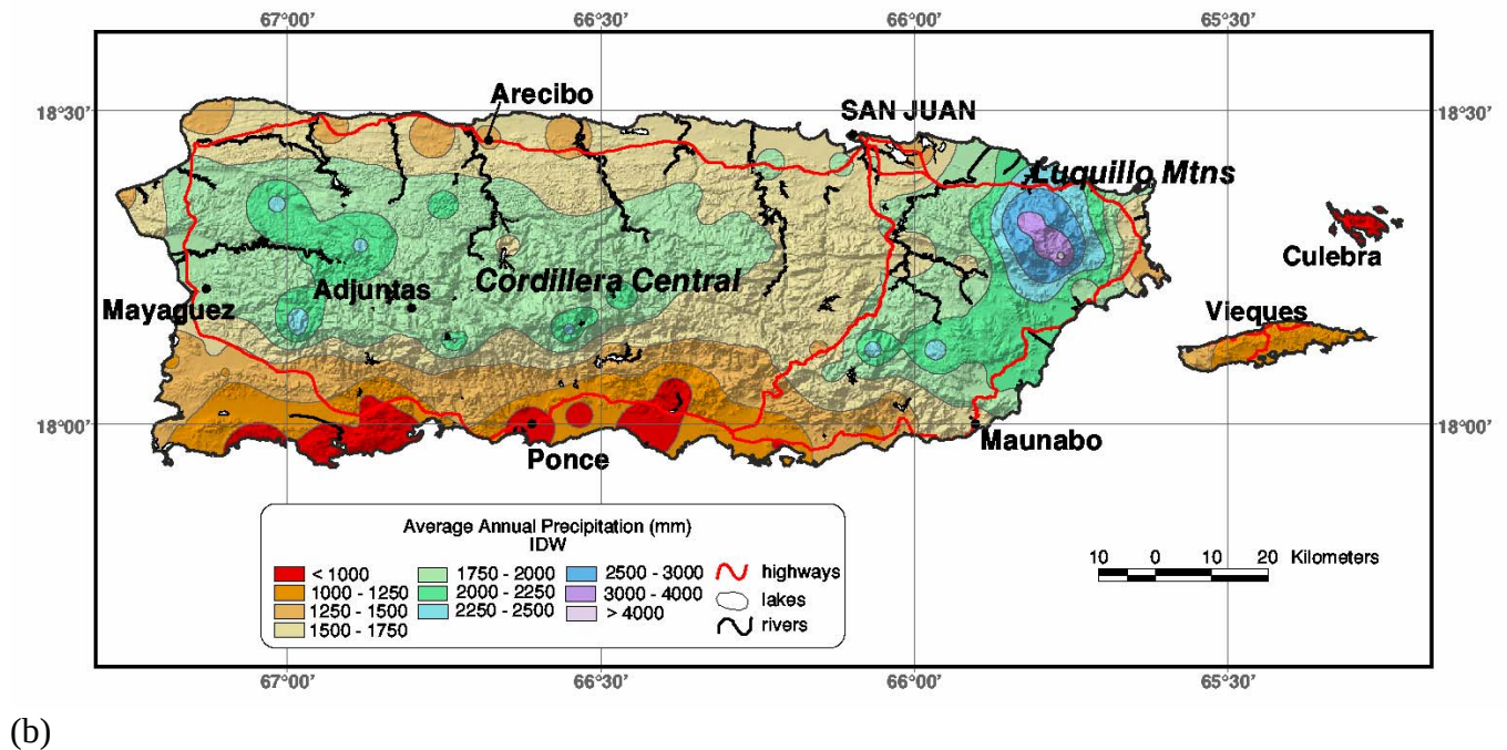
(b) Figure 10. Mean 1963-95 annual precipitation for Puerto Rico, Vieques, and Culebra: (a) PRISM; (b) IDW
