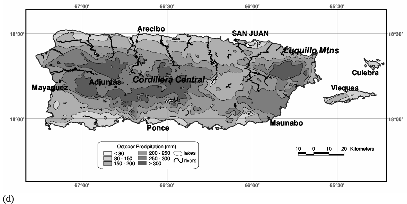
Figure 9 (Continued) Mean 1963-95 in (c) July; (d) October for Puerto Rico, Vieques, and Culebra; PRISM parameterization
