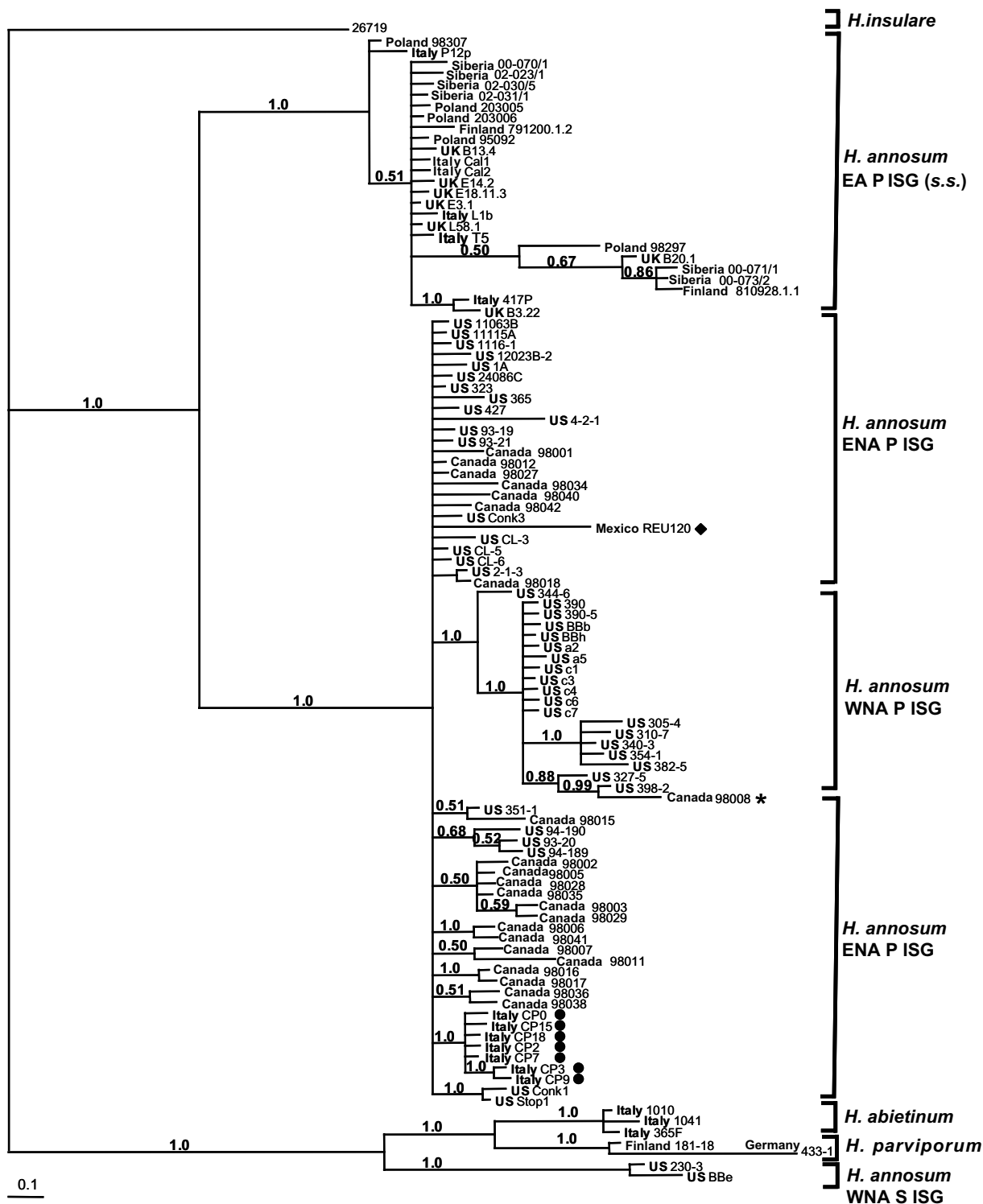
Fig. 5. Fifty-percent majority-rule phylogram of Bayesian analysis of partitioned, multilocus dataset: GPD, EFA and ATP. Calculations made with entire dataset; data divided into four partitions—standard, for indel data, and three different gene regions for the DNA sequence data. Posterior probabilities larger than 0.5 from 1,000,000 generations of Bayesian analysis are shown above the branches. Isolates from Castelporziano are marked with filled circles, the Mexican isolate with a filled diamond. WNA, western North America; ENA, eastern North America; EA, Eurasia. Outgroup is H. insulare . *Clade placement of ENA isolate 98008 incongruent with geographic origin.
