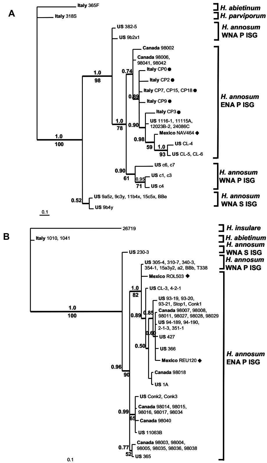
Fig. 4. Fifty-percent majority-rule phylogram of Bayesian analysis of 1.6 and 1.8 kb insertions into the mitochondrial ML5–ML6 region of rDNA. Partial, concatenated sequence. Thickest bold branches were supported in strict MP and 50% Bayesian consensus trees. Thinner bold branches were supported in only one type of consensus tree. Bootstrap values of 50 and above from 1000 replicates for MP analysis shown below the branches; posterior probabilities 0.5 or larger from 1,000,000 generation Bayesian analysis shown above the branches. Isolates from Castelporziano (CP) are marked with a filled circle, the Mexican isolates, with a filled diamond. WNA, western North America; ENA, eastern North America; EA, Eurasia. (A) 1.6 kb insertion. Outgroup is H. abietinum . (B) 1.8 kb insertion. Outgroup is H. insulare .
