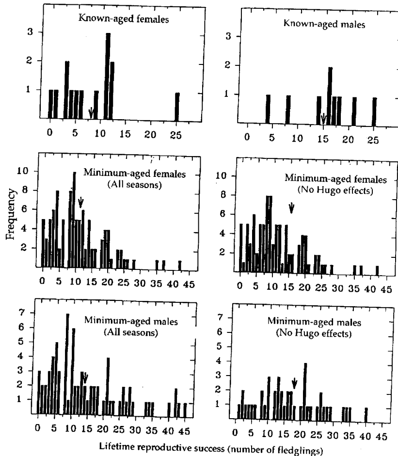
Figure 3. -Lifetime reproductive success (expressed as number of fledglings) in known- and minimum-aged pearly-eyes. Breeding success was compared excluding the effects of Hurricane Hugo by eliminating the 1990 and 1991 breeding seasons. Although frequency distributions are visually altered, they are not significant for either sex at the 95 percent level of confidence. Arrows (↓) are means.
