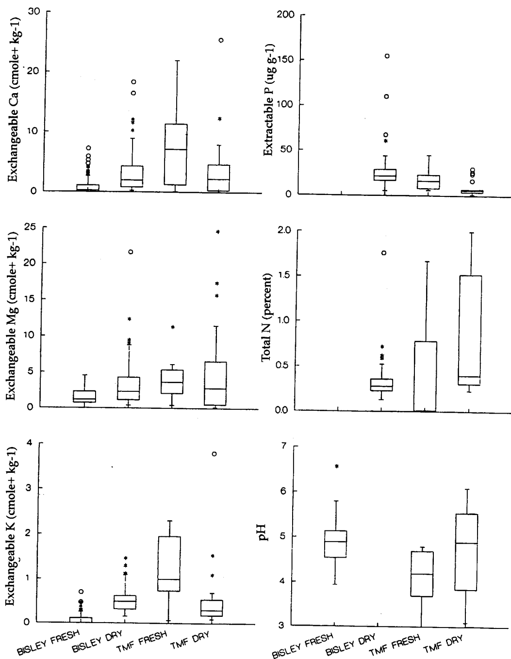
Figure 1. -Box plots of the range of values of nutrient concentrations in surface soils (0-10 cm) of the Bisley Research Watersheds, Luquillo Experimental Forest, Puerto Rico, and other tropical montane forest (TMF) sites combined. Data sets using fresh soils (Bisley Fresh, TMF Fresh) and dry/ground soils (Bisley Dry, TMF Dry) are compared. Bars represent the median between the whiskers; boxes enclose the interquartile range; stars represent outliers, and dots are far outside values (Silver et al. 1994).
