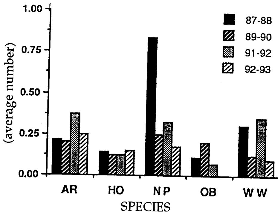
Figure 1. -Abundance of five species of winter-resident warblers on St. John, U.S. Virgin Islands. Average number of individuals per survey point in moist forest ( n=40 ) for the following species: American redstart (AR), hooded warbler (HO), northern parula (NP), ovenbird (OB), and black-and-white warbler (WW).
