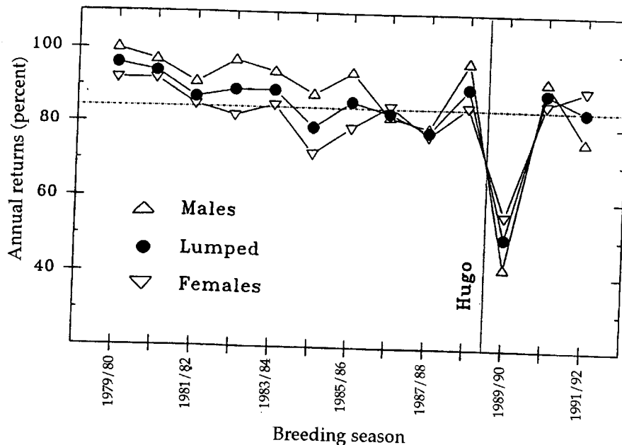
Figure 1. -Annual return rates of 86 male and 121 female pearly-eyed thrashers breeding in nest boxes between 1979 and 1992. Hurricane Hugo significantly lowered return rates, but predisturbance levels were recouped by the second breeding season following disturbance. The plot-wide dot-dashed line is the mean return rate for both sexes.
