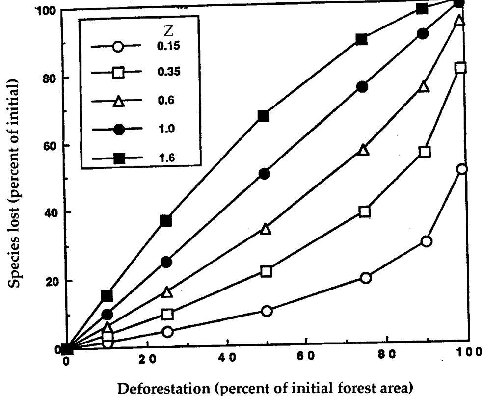
Figure 1. -Relationship between deforestation and loss of species to extinction using different slopes (Z factor) for the species-area curve.
