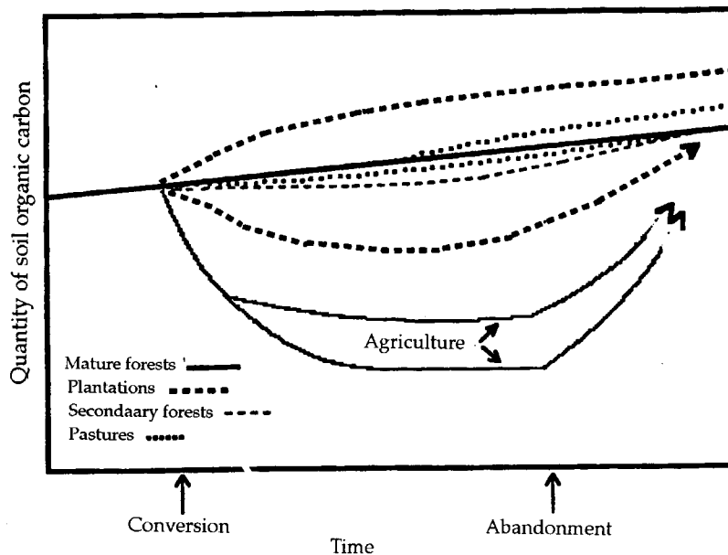
Figure 3. -Suggested patterns of change of soil organic carbon in soil subjected to different land uses in the Tropics. This model ignores variations due to soil type and mechanical conversions of sites. The type of agricultural use or plantation species planted changes the slope of the curves (Lugo and Brown 1992).
