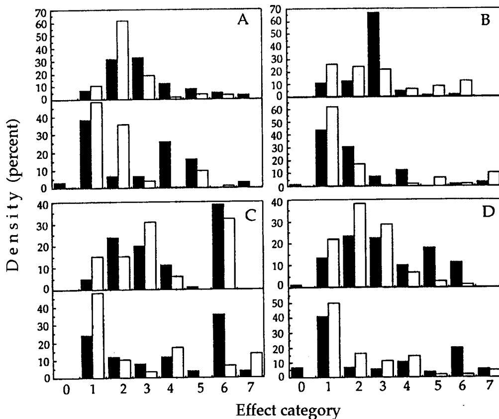
Figure 2. -Effects distribution by diameter classes expressed in the percent of total tree density for Guzmán (A), Cubuy (B), Sabana (C), and El Verde (D) areas in the Luquillo Experimental Forest. Black and white bars represent plantation and secondary forest plots, respectively. Trees d.b.h. \geq 10 cm, superior graph, and trees with a d.b.h. < 10 cm, inferior graph. See table 1 for effect definitions.
