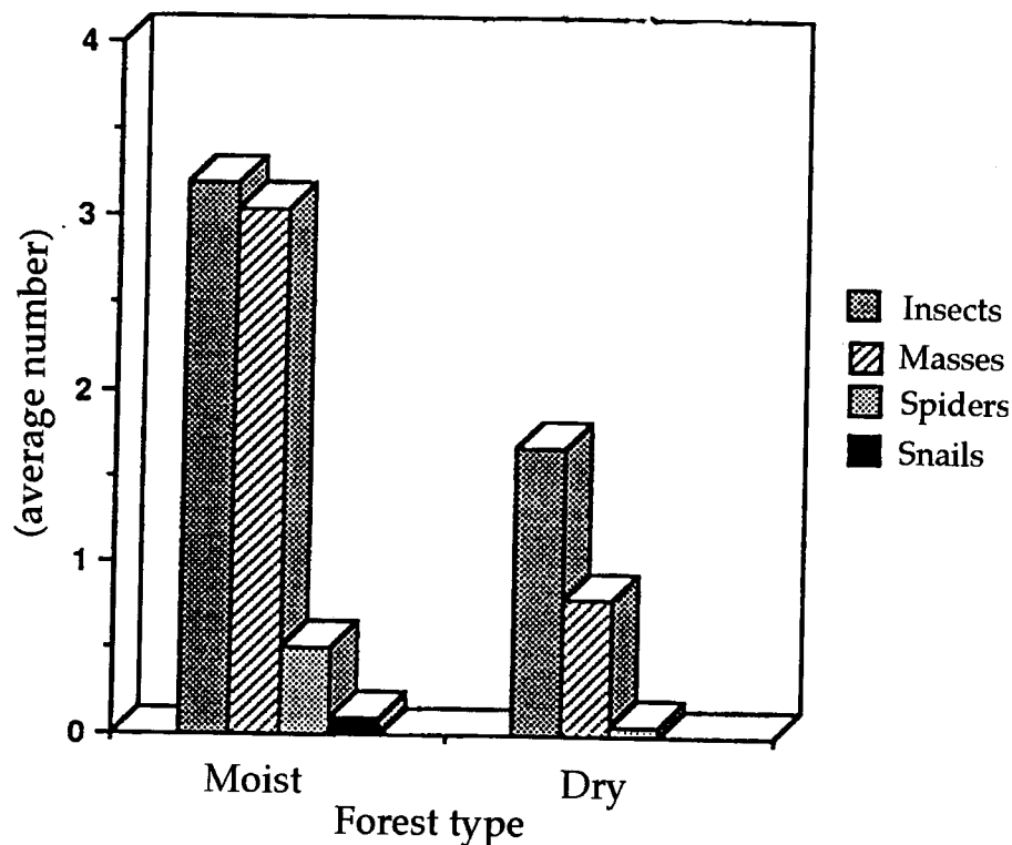
Figure 3. -Average number of individuals (for insects, spiders, and snails) or masses of individuals (aggregations of eggs or tiny insects such as aphids or mealy bugs). Average are for six transects in moist forest (moist) and three transects in dry woodland (dry) that were surveyed in a preliminary study.
