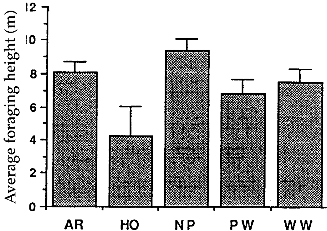
Figure 2. -Average foraging heights for the five species of warblers most frequently observed in a preliminary study: American redstart (AR), hooded warbler (HO), northern parula (NP), prairie warbler (PW), and black-and-white warbler (WW). Sample sizes are as follows: American redstart - 30, hooded warbler - 6, northern Parula - 33, prairie warbler - 10, black-and-white warbler - 23. Error bars indicate standard errors.
