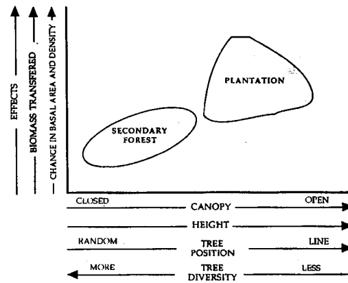
Figure 4. -Comparison of a typical structure of a plantation and its response to the hurricane with its paired secondary forest (adapted from Rodríguez Pedraza 1993).
