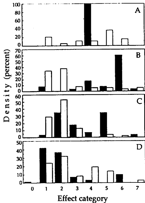
Figure 3. -Hurricane effects expressed in percent of total tree density for the species Schefflera morototoni (A), Miconia prasina (B), Tabebuia heterophylla (C), and Casearia arborea (D) in plantation plots (black) and paired secondary forests (white), Luquillo Experimental Forest. See table 1 for effects definitions.
