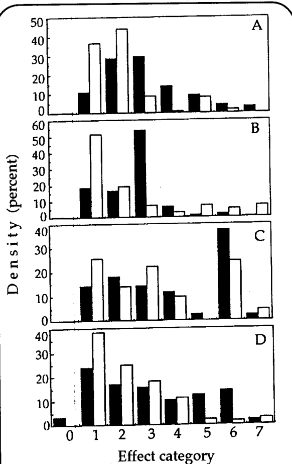
Figure 1. -Hurricane effects expressed in percent of total tree density for the plots of Guzmán (A), Cubuy (B), Sabana (C), and El Verde (D) in the Luquillo Experimental Forest. Black and white bars represent plantation and secondary forest plots, respectively. See table 1 for effect definitions.
