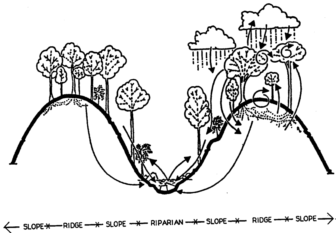
Figure 5. -Model of nutrient cycling in a subtropical wet forest in Puerto Rico (Lugo and Scatena 1992). Arrows illustrate the fluxes of nutrients and organic matter and define interfaces where organisms interact with the abiotic environment (table 4).
