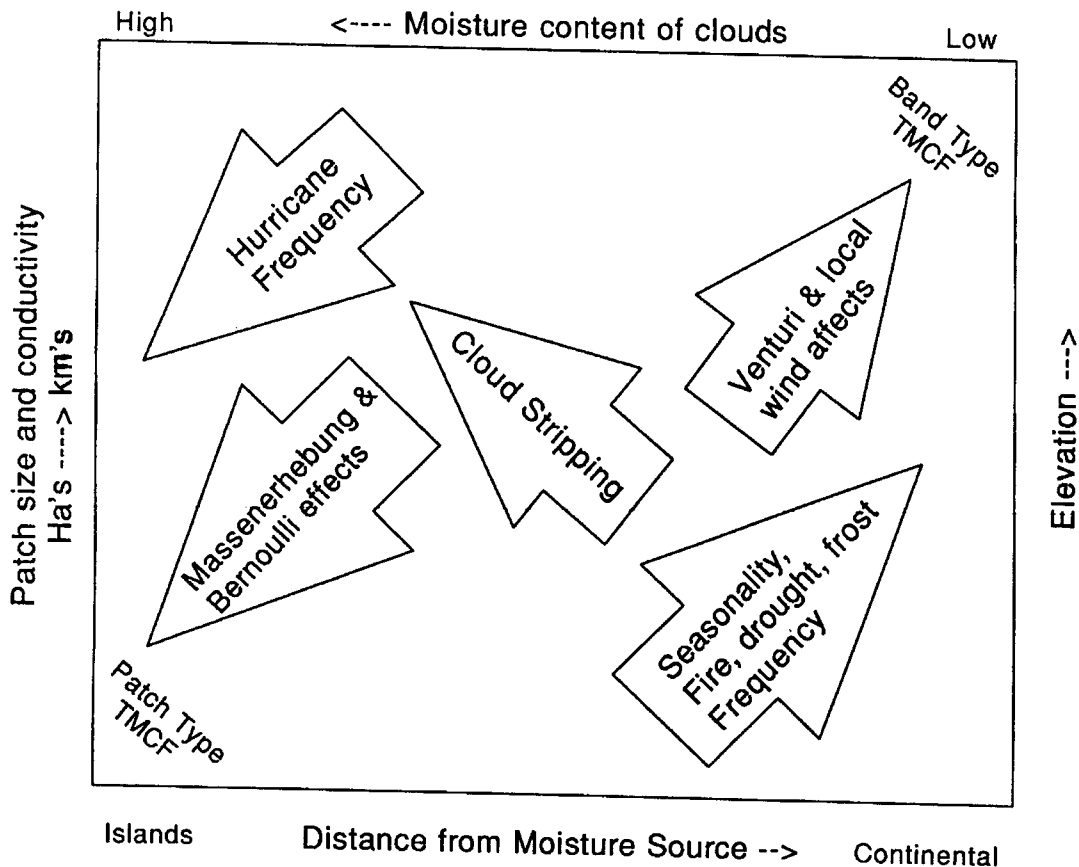
Figure 1. -Conception of the relationships of various ecosystem properties that influence tropical montane cloud forests. Arrows indicate direction of increasing importance of system property (Hamilton, Scatena, and Juvik 1993).
