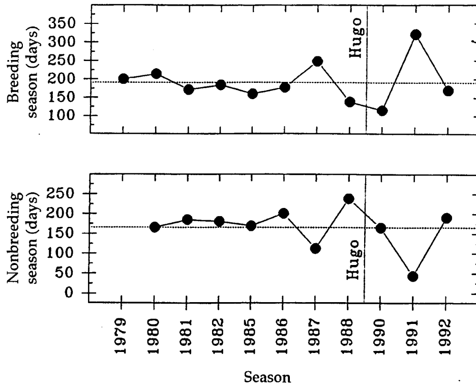
Figure 2. -Lengths of 11 pearly-eyed thrasher breeding and nonbreeding seasons. The plot-wide horizontal dashed lines are the overall average lengths of all breeding and nonbreeding seasons sampled between 1979 and 1992. The effects of Hurricane Hugo were significant on the length of both breeding and nonbreeding seasons.
