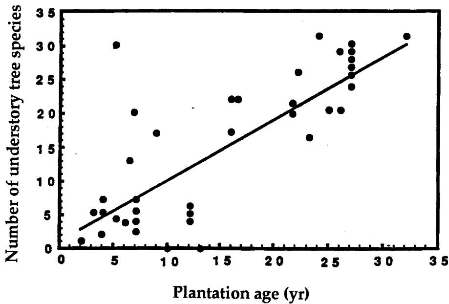
Figure 2. -Relationship between number of understory tree species in tree plantations and the age of the plantation (Lugo et al. 1993). The relationship for these data is y=0.74+ 0.93 x , ( r^2 = 0.62 ).
