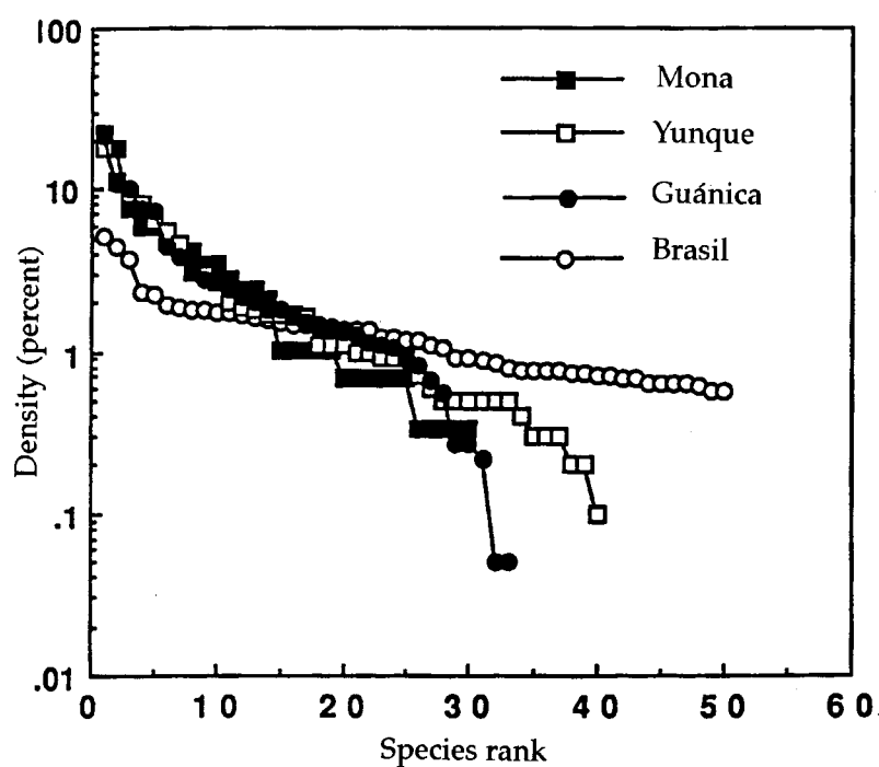
Figure 9. -Relative Importance curves for the most diverse community on Mona Island (lowland forest), a mature semideciduous forest in Guánica, the Luquillo Experimental Forest, and a moist forest in the Amazon basin of Brazil (Lugo 1991).
