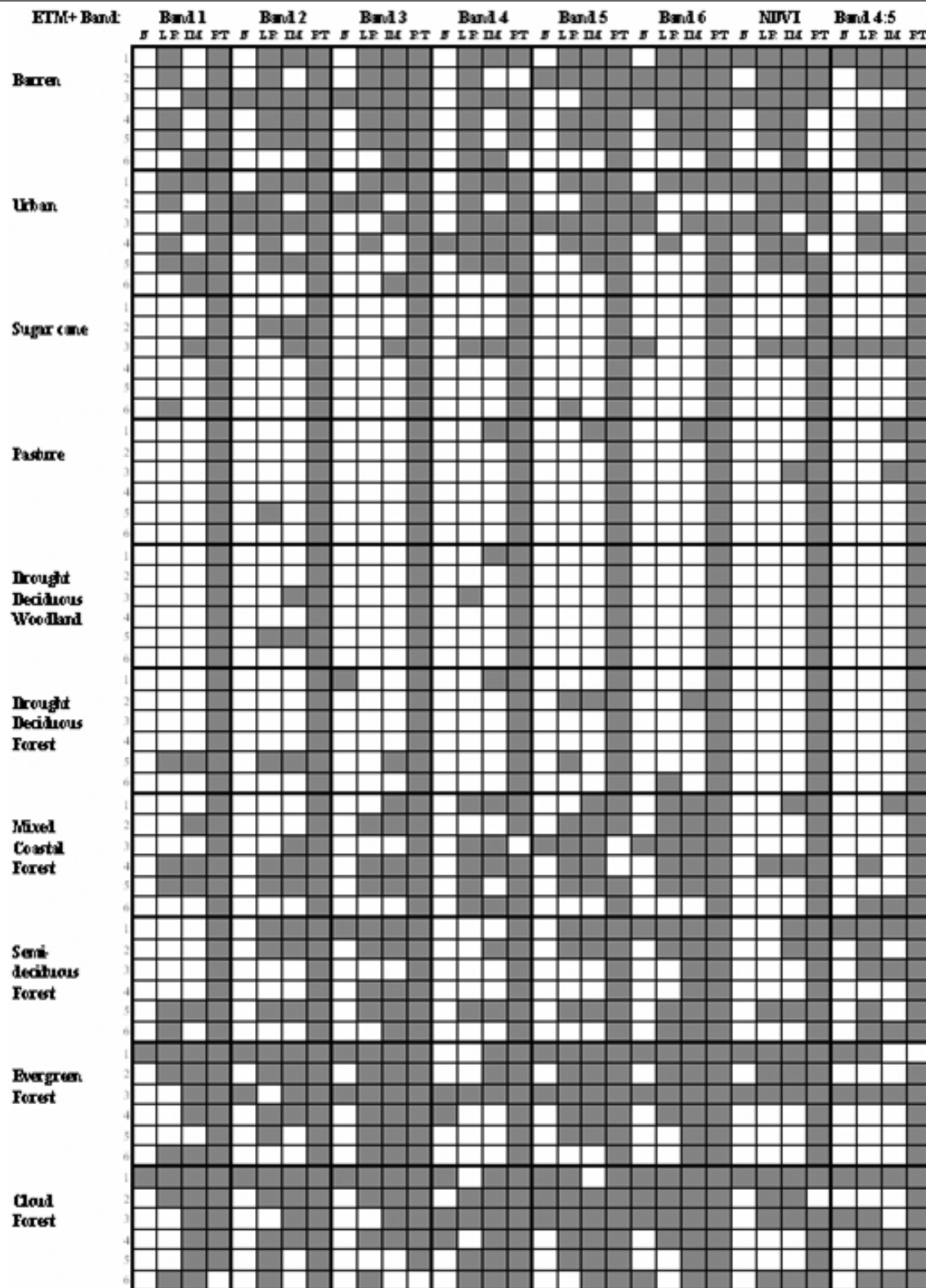
Figure 2. Results from 480 ANOVAs to compare normalization results. Each square outlined by a bold line shows results for one band and one class for each of six separate multiple comparisons of means (MCMs). The six MCMs result from the six reference–subject image pairs that fill clouds in the two cloud-filled images in Figures 4 and 5 (three pairs for the leaf-on imagery in Figure 4 and three pairs for the leaf-off imagery in Figure 5 ). The four small columns in each bold-outlined square are the four explanatory variable conditions: no normalization or correction (N), linear regression normalization (LR), image match histogram matching (IM), or regression tree normalization (RT). Shaded squares indicate which conditions yielded the smallest significantly different group of means for each MCM (for the particular band, class, and reference–subject image pair). Reference–subject scene pairs 1–6 are as follows: 1, 11 Sept. 2002 – 2 Feb. 2003; 2, 11 Sept. 2002 – 5 Sept. 2000; 3, 11 Sept. 2002 – 12 Dec. 1999; 4, 12 Dec. 1999 – 2 Feb. 2003; 5, 12 Dec. 1999 – 5 Sept. 2000; 6, 12 Dec. 1999 – 11 Sept. 2002.
