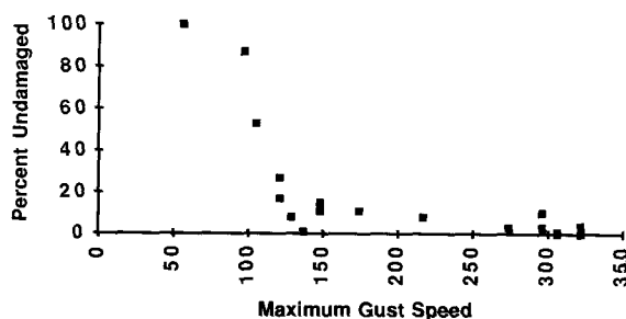
Figure 2. Percentage of all trees surveyed receiving no damage plotted against maximum gust speed.
