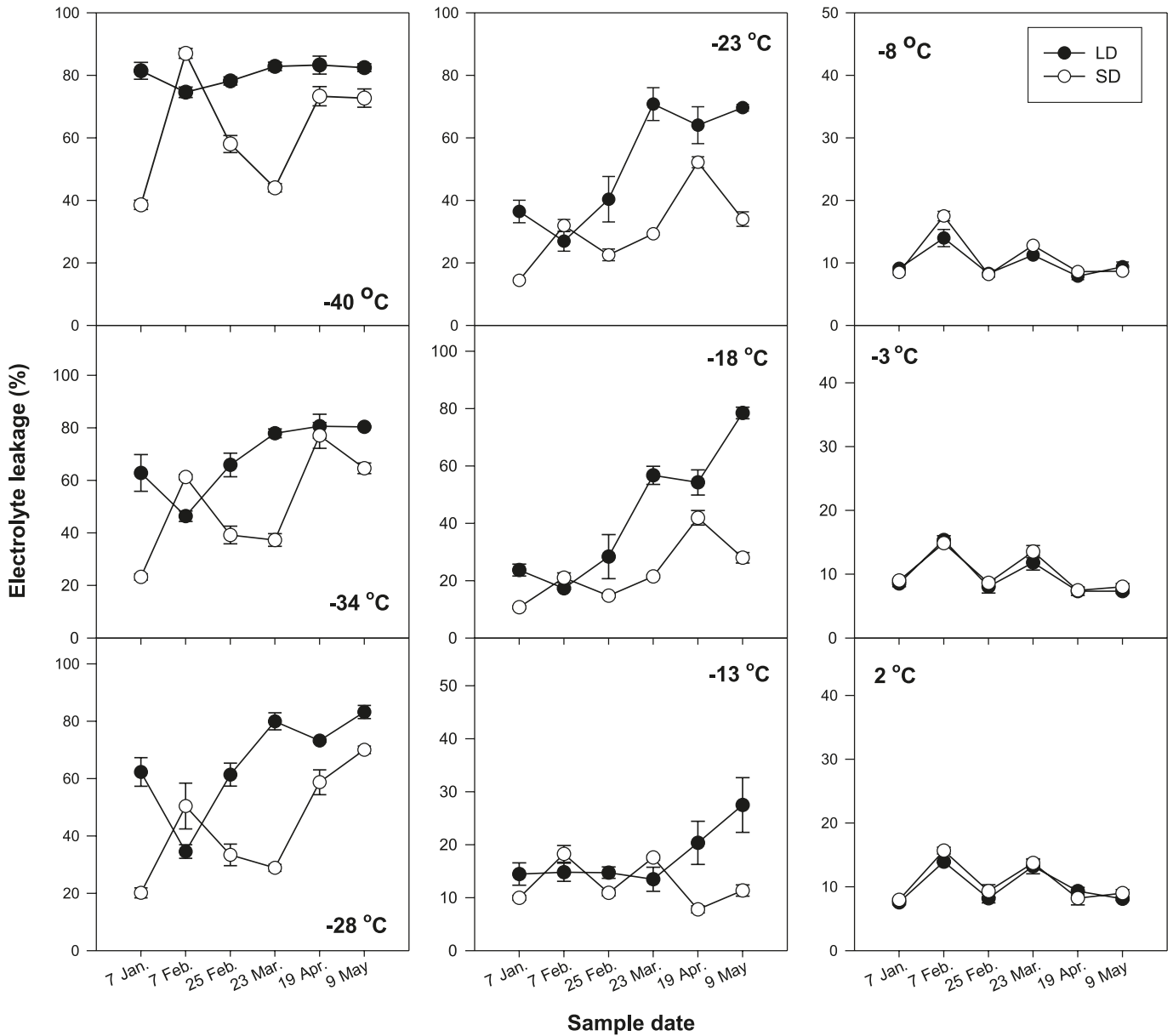
Fig. 1. Mean ( \pm SE) electrolyte leakage values for each freezing test temperature across sampling dates for either ambient (long-day (LD)) or midsummer short-day (SD) photoperiod treatments.
