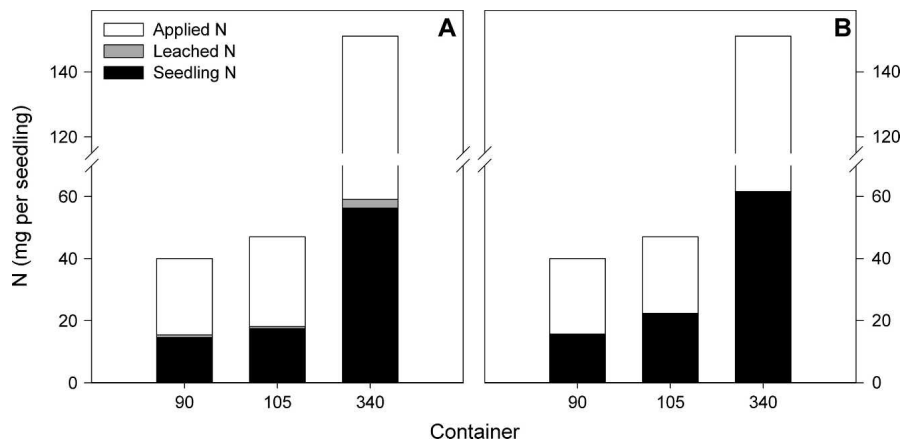
Fig. 1. Applied, leached, and seedling nitrogen values for overhead-irrigated coneflowers (A) and subirrigated coneflowers (B).
