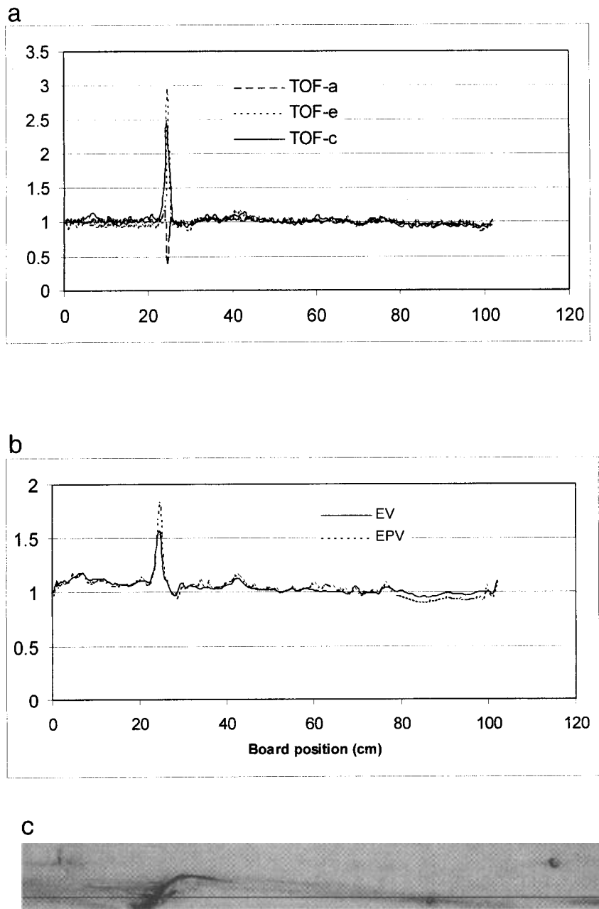
FIG. 7. Normalized ultrasonic variables are graphed for a scan line through a bark pocket in a yellow-poplar deckboard, (a) TOF-a, TOF-e, and TOF-c, (b) EV and EPV, and (c) board photo. The scan line is marked on the board image.
