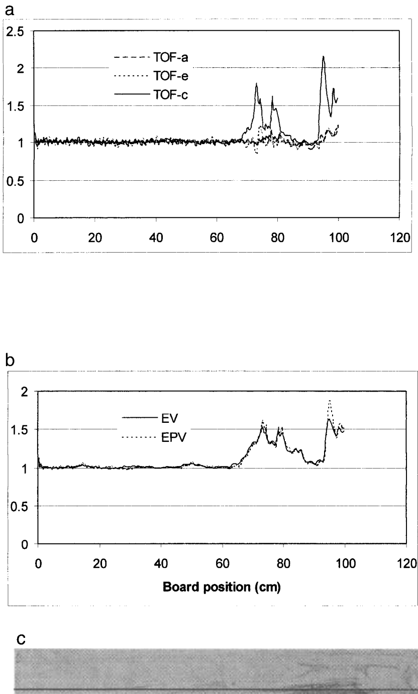
FIG. 8. Normalized ultrasonic variables are graphed for a scan line through decay in an oak deckboard, (a) TOF-a, TOF-e, and TOF-c, (b) EV and EPV. The scan line is marked on the board image.
