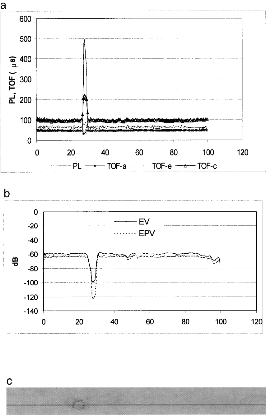
FIG. 5. Ultrasonic variables are graphed for a scan line through an unsound knot in red oak, (a) energy, PL, TOF-a, TOF-e, and TOF-c, (b) EV and EPV, and (c) board photo. The scan line is marked on the board image.
