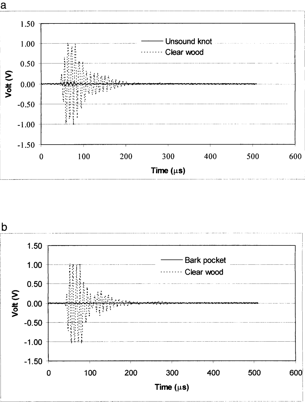
FIG. 3. Ultrasonic time-domain signals through clear and effected yellow-poplar show a dramatic loss in signal strength for unsound defects, (a) an unsound knot, (b) bark pocket.
