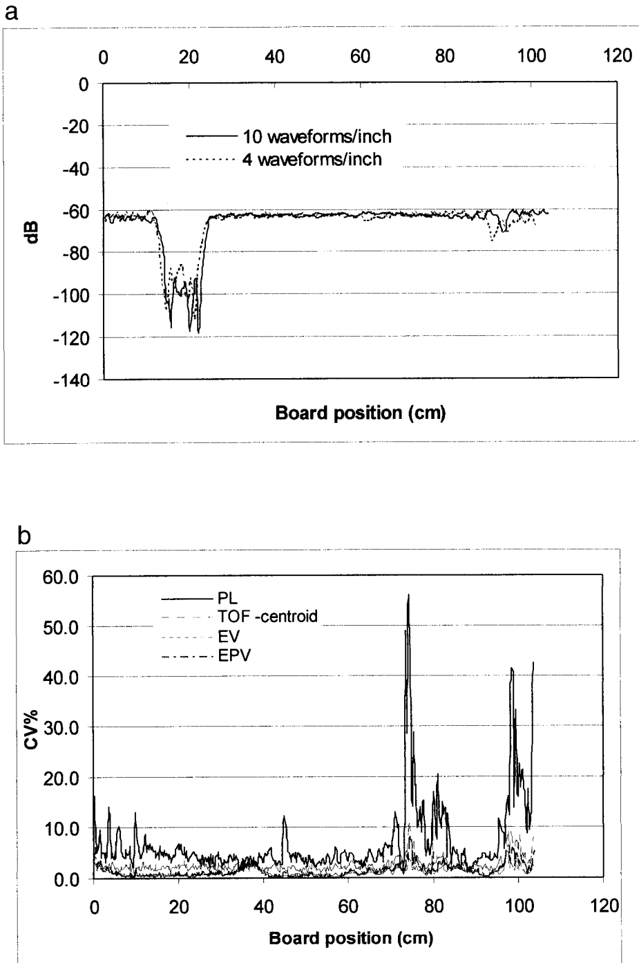
FIG. 11. Energy loss values are plotted for two different scanning rates along the same scan line on a red oak board (a). Percent coefficient of variation (CV%) is shown for several ultrasound variables using ten repeated measurements of the same scan line on a yellow-poplar board (b).
