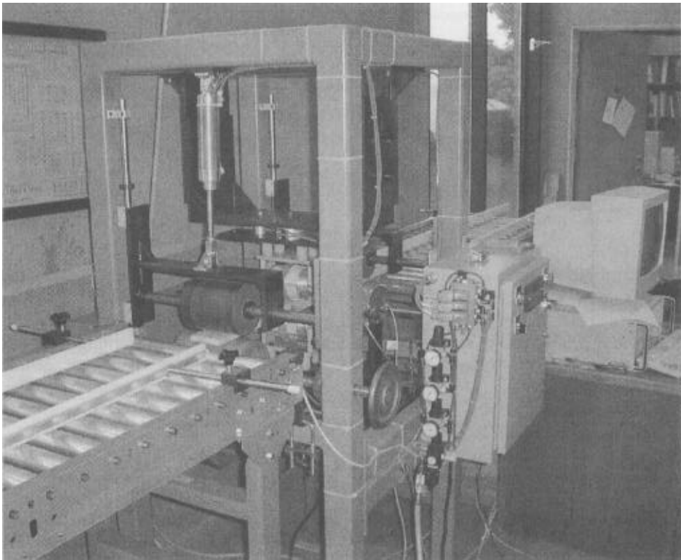
FIG. 2. Our ultrasonic scanning system includes materials handling, computer control of part movement and data collection, and ultrasound electronics.
