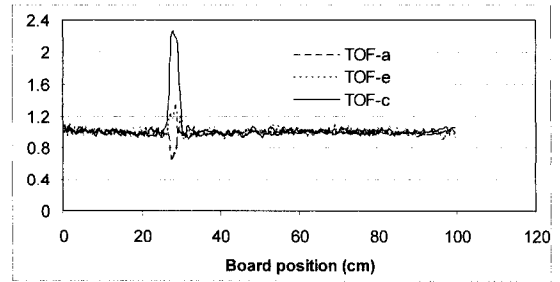
FIG. 6. Normalized TOF-a, TOF-e, and TOF-c, values are plotted for the deckboard in Fig. 5c.
