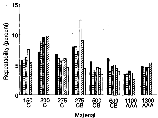
FIG. 3 — Repeatability coefficient of variation for eight materials after various postwaxing reconditioning times and for four materials in Sumitomo fixture.
