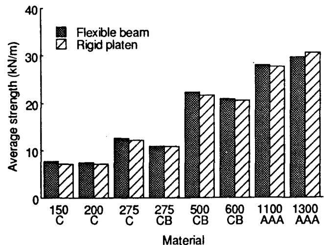
FIG. 8 — Average observed edgewise compressive strength of eight materials tested in flexible-beam loading machine and predicted average strength of materials tested in rigid-platen machine.
