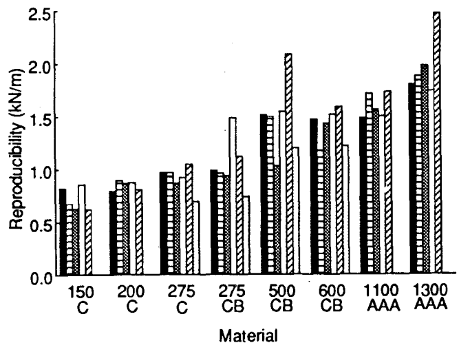
FIG. 4 — Reproducibility standard deviation ( S_R ) for eight materials after postwaxing reconditioning times and for four materials in Sumitomo fixture.
