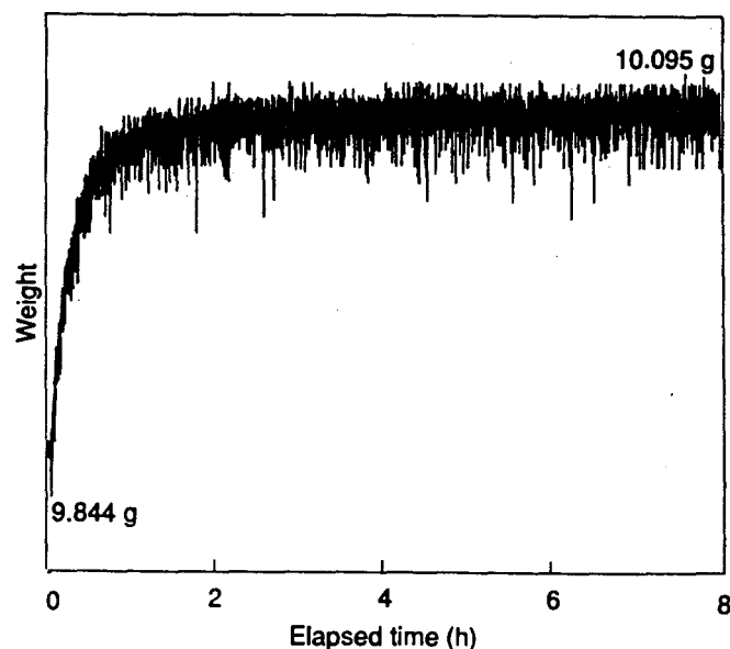
FIG. 11 — Weight of corrugated fiberboard short column specimens as a function of time in a 23°C (73°F), 50% RH conditioned room with forced air circulation after removal from a 27°C (80°F), 30% RH preconditioning room.
