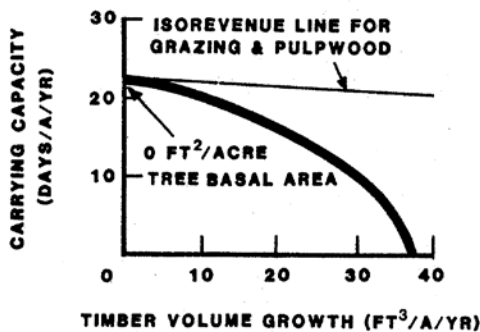
Figure C.--Optimum thinning intensity when considering grazing and current pulpwood prices.
