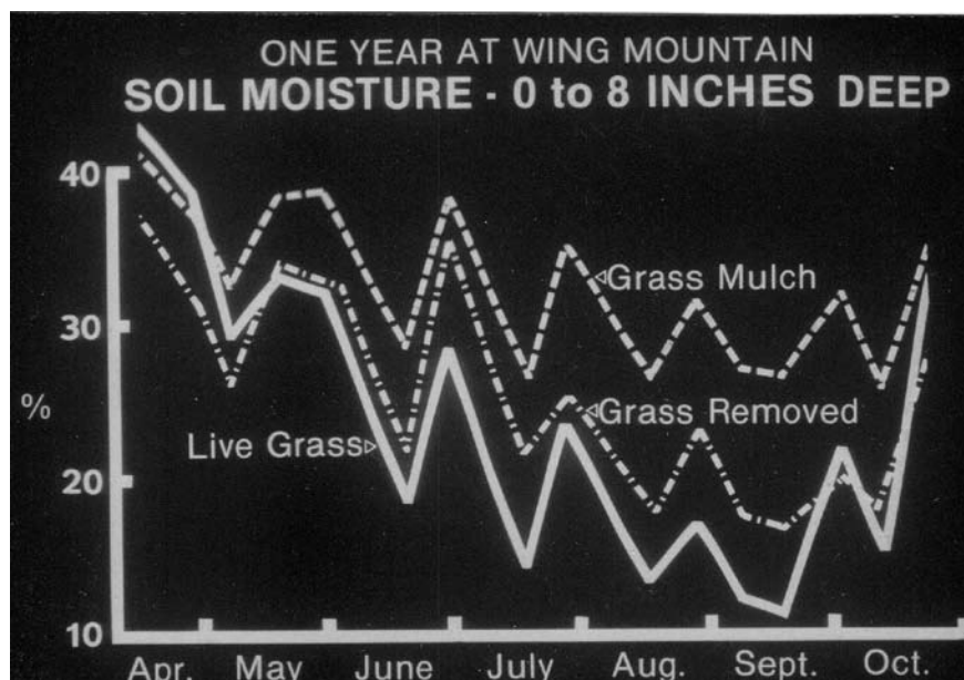
Figure 9. Soil moisture at Wing Mountain, AZ for 0 to 20- cm depth comparing moisture on plots with dead grass, grass removed, and live grass, in 1963.
