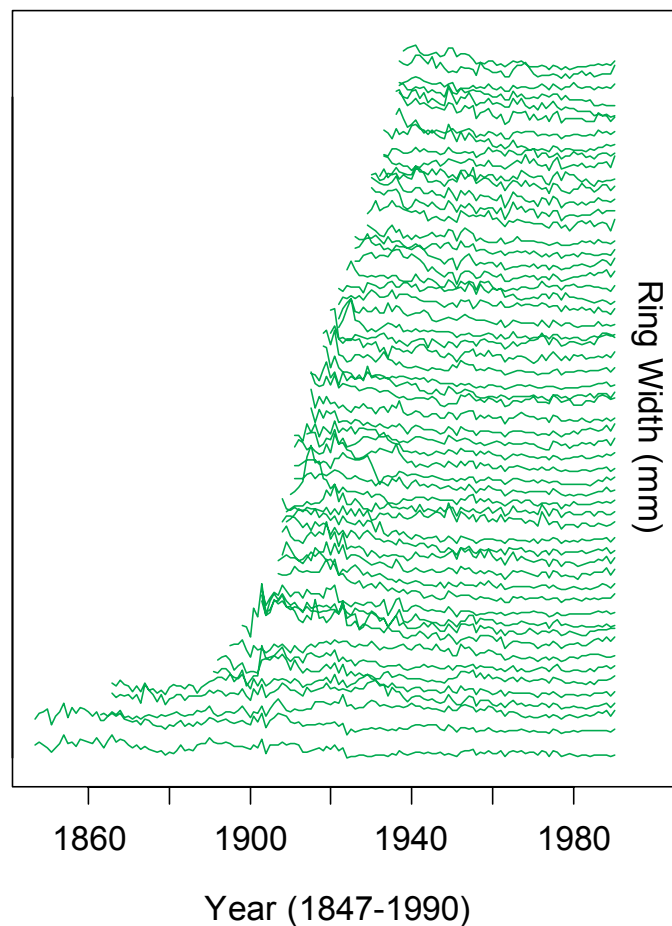
Figure 2. Time-series plots of ring-width measurements, sorted by first year, from wood increment cores taken at the G.A. Pearson Natural Area, Arizona, U.S.A. (see text for details). The vertical scale (not shown) was the same for all segments. Ponderosa pines with DBH > 50 cm Ponderosa pines with DBH < 50 cm
