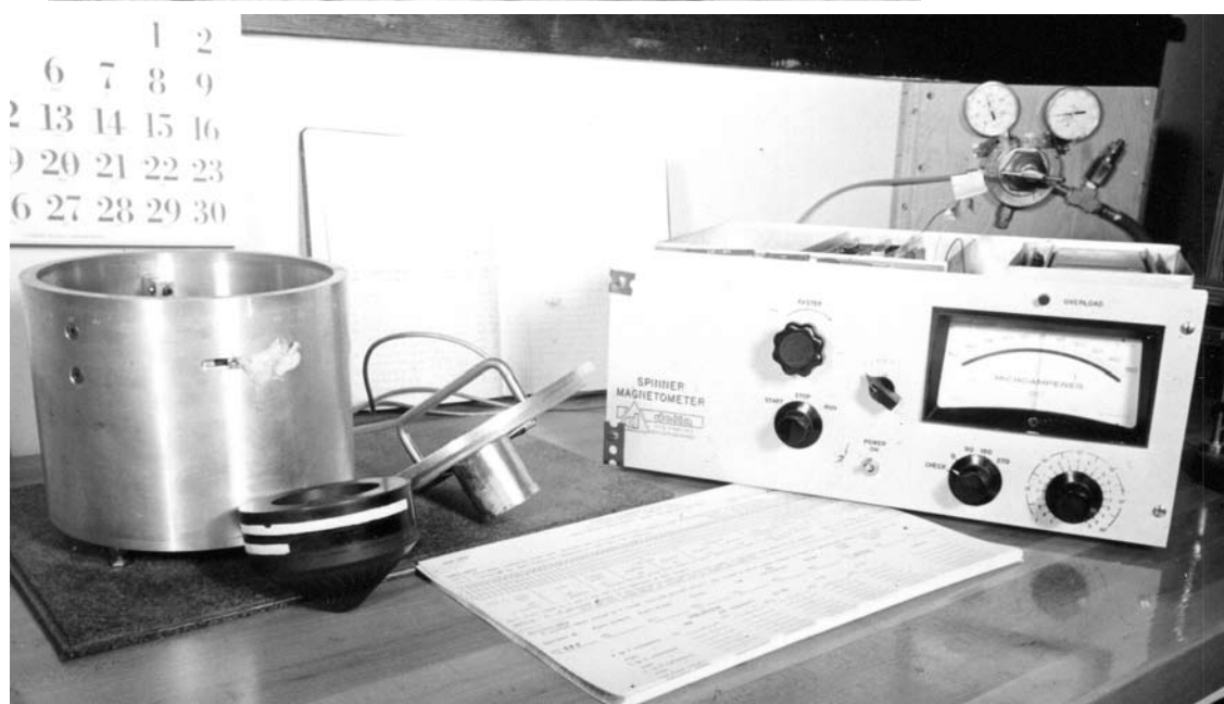
Figure 4. Spinner magnetometer.
