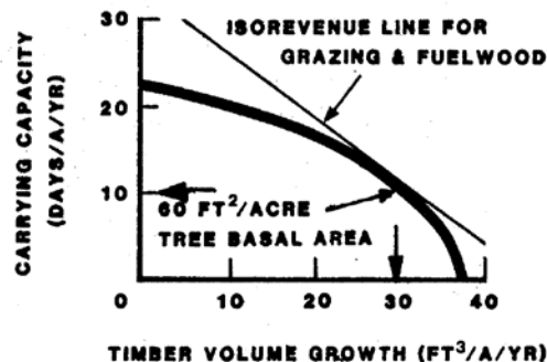
Figure D.--Optimum thinning intensity when considering grazing and current fuelwood prices.
