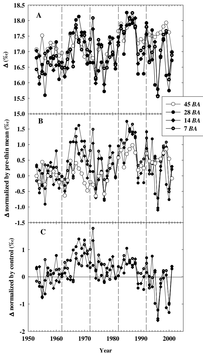
Figure 4. A) Carbon isotope discrimination ( \Delta ), B) \Delta nominalized to prethinning (1952-1961) \Delta , and C) \Delta nominalized to the unthinned control for the 45, 28, 14 and 7 m^2 ha^{-1} basal area treatments for years 1952-2001. Each point represents a plot mean value obtained by pooling five trees per plot into a single sample. The initial thinning treatment (1962) and subsequent thinning treatments (1972, 1982, 1992) are indicated by the vertical dashed lines. From McDowell et al. (2006).
