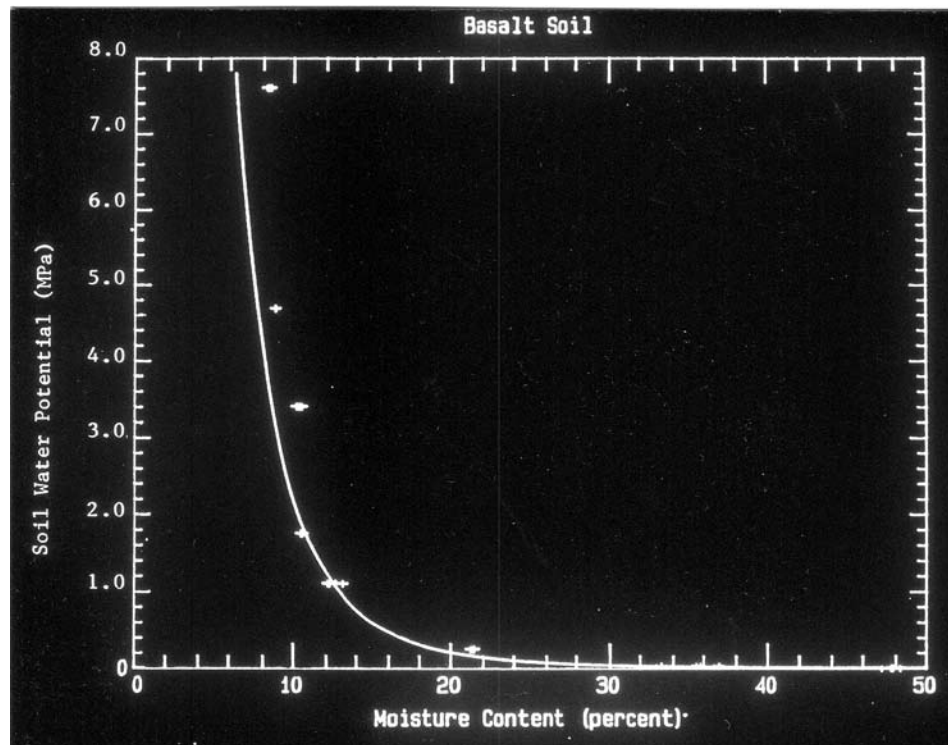
Figure 4. Soil moisture content (%) plotted against soil water potential in megapascals (Mpa) for a basalt soil in northern Arizona. One Mpa roughly equals ten bars of atmospheric pressure. Below 10% SMC water becomes more limiting for ponderosa pine seedlings.
