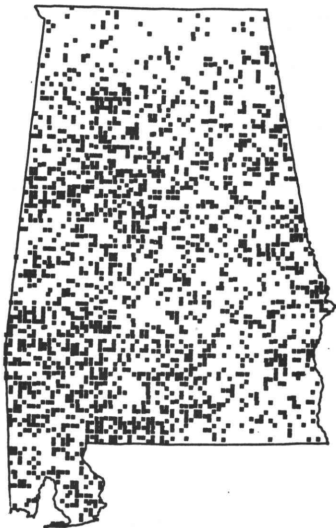
Figure 3.—Distribution of softwood biomass, each dot representing 300,000 tons woody green weight.
