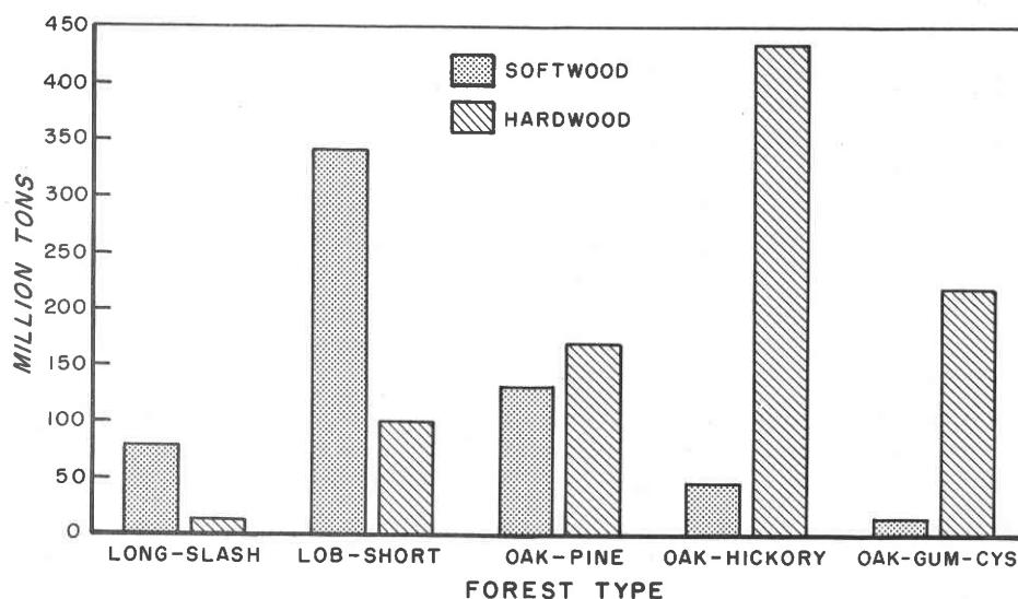
Figure 11.—Woody biomass by major forest type in Alabama.
