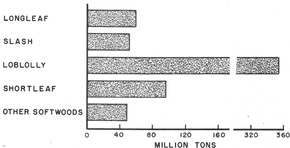
Figure 7.—Softwood woody biomass by species in Alabama.
