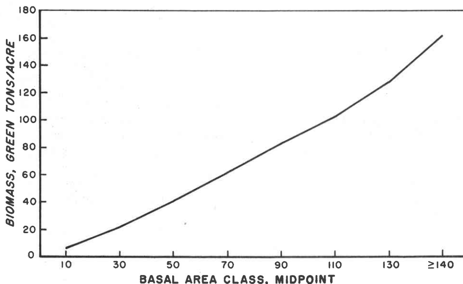
Figure 8.—Relationship of woody biomass to basal area in Alabama.
