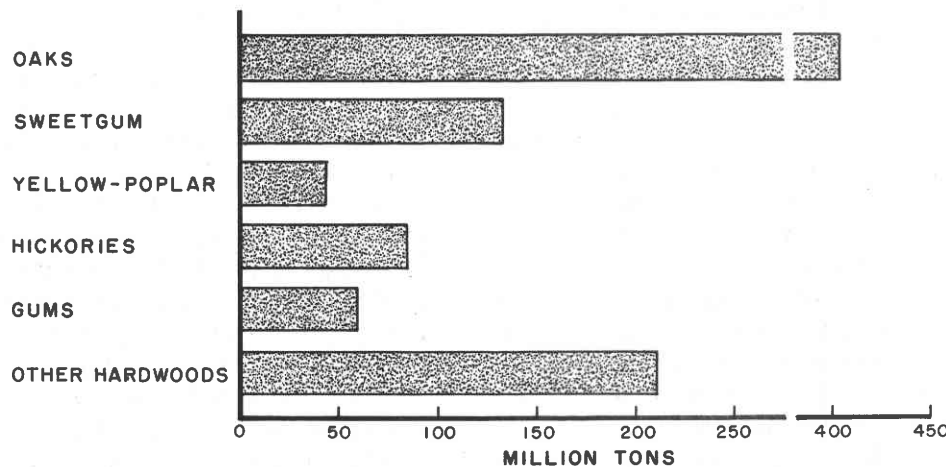
Figure 6.—Hardwood woody biomass by species in Alabama.
