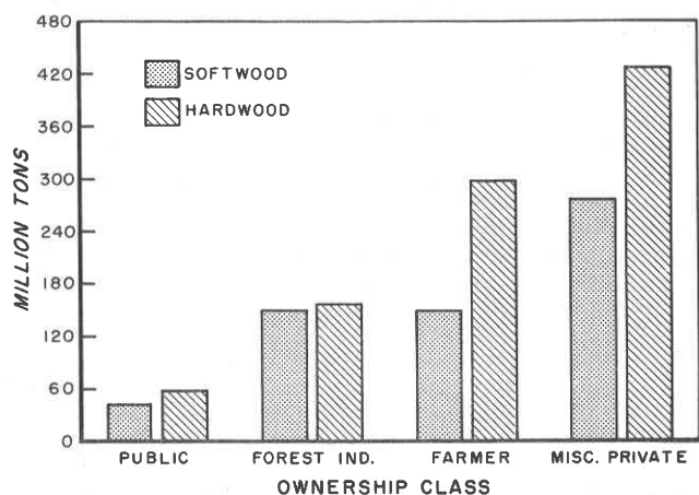
Figure 10.—Woody biomass by major ownership category in Alabama.
