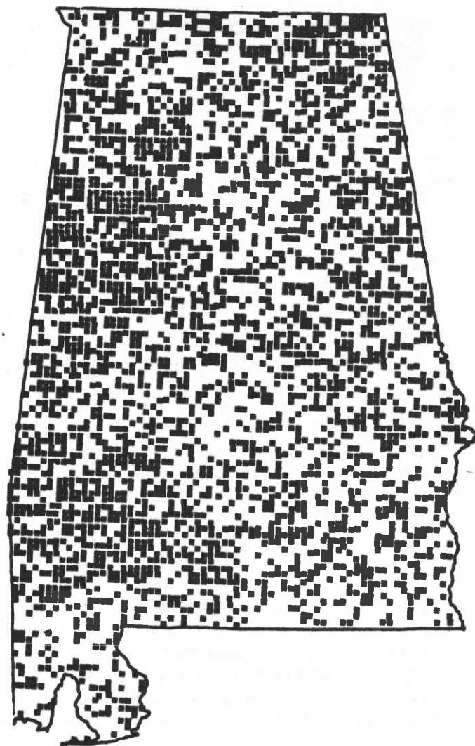
Figure 4.—Distribution of hardwood biomass, each dot representing 300,000 tons woody green weight.
