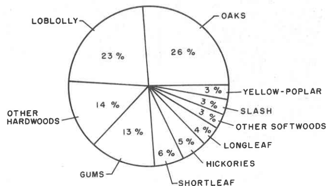
Figure 5.—Percent of total Alabama woody biomass by species.
