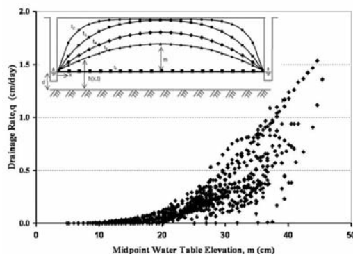
Figure 1. Measured drainage rate, q , and water table elevation above water level in ditch, m , during 1996 for a Bellhaven muck on the Parker Tract, Washington County, North Carolina. Inset shows evolution of predicted water table shape with time after rainfall ceased at time, t_2 .
