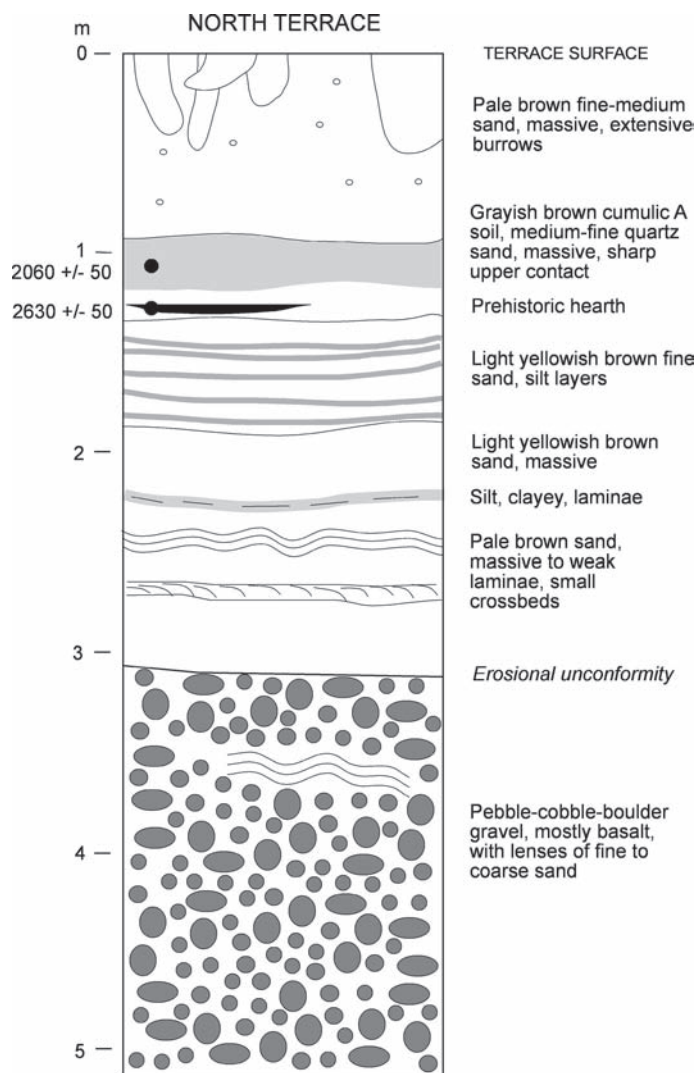
FIGURE 7. North terrace alluvial stratigraphy; see photo in Fig. 3; the dated prehistoric hearth occurs downstream and is physically correlated to the level shown; the single cumulic paleosol correlates to paleosol F in the south terrace sequence (Figs. 4, 5).
