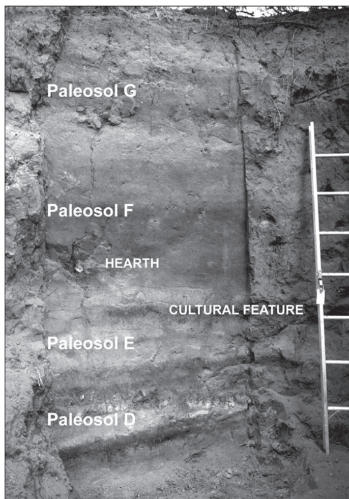
FIGURE 4. South terrace fine sand alluvium with four cumulic A paleosols and prehistoric cultural features; section shown is approximately 300 cm thick and is the upper portion of the south terrace sequence.
