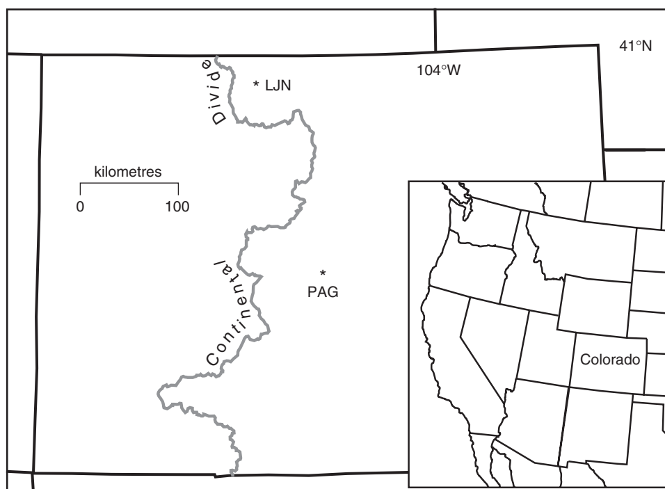
Fig. 1. Location map of sites Lake John (LJN) and Packer Gulch (PAG) in Colorado.
