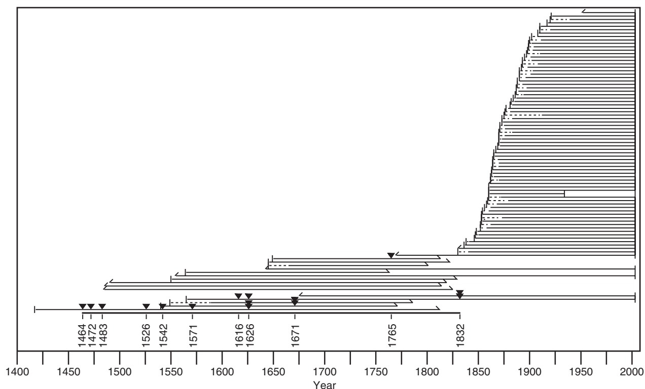
Fig. 2. Tree-recruitment and fire-scar chronology from Lake John (LJN). Only limber pine were sampled at the site. Horizontal lines mark time spans of individual trees with dates of fire scars marked by inverted triangles. Dashed lines are estimated number of years to pith dates on cores or cross-sections that did not intersect pith but inside ring curvature was visible. Vertical lines to left on each tree chronology are pith dates with inside dates (i.e. unknown number of years to pith) marked by slanted lines. Vertical lines to right are bark dates (= death dates in remnant trees) with outside dates (i.e. unknown number of years to death date) marked by slanted lines. Top tree chronologies are from plot trees, with additional trees collected for fire scars at the bottom (see Methods).
