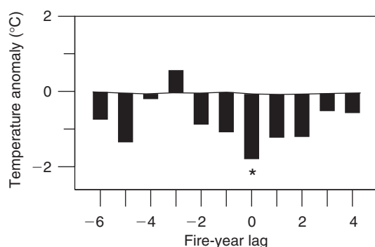
Fig. 6. Superposed epoch analyses of average summer temperature anomalies in northern Colorado (C. Woodhouse, P. Brown and M. Hughes, unpubl. data) for Lake John (LJN) fire years listed in Fig. 1. Fire year lag '0' is the average climate anomaly for fire years, with antecedent conditions indicated by negative lags. Asterisk marks significant departure in average climate conditions based on bootstrapped confidence intervals ( P < 0.05 ).
