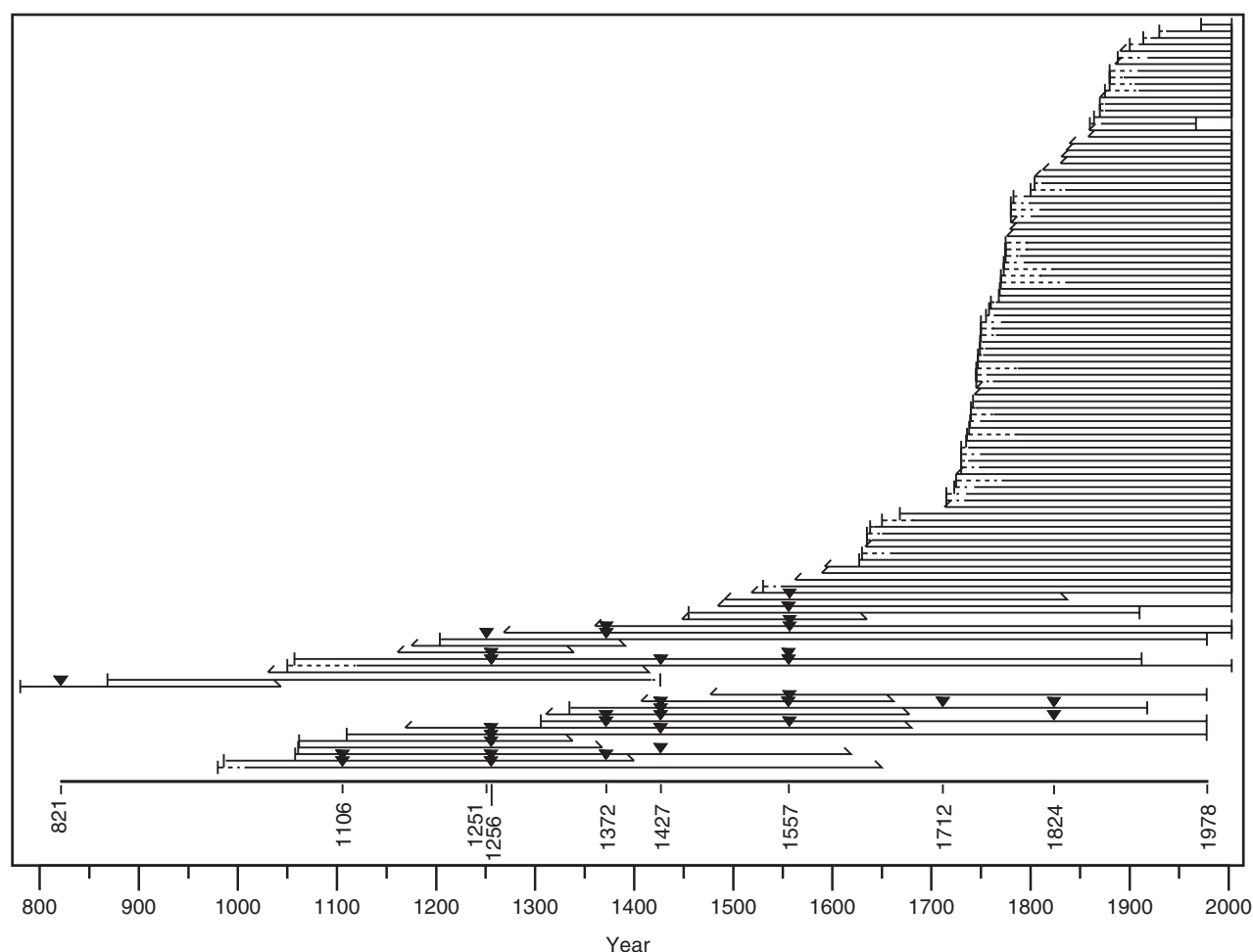
Fig. 3. As in Fig. 2 for trees collected at Packer Gulch (PAG). Graph includes all species sampled at the site, including Rocky Mountain bristlecone pine, limber pine, Engelmann spruce, and Douglas-fir.
