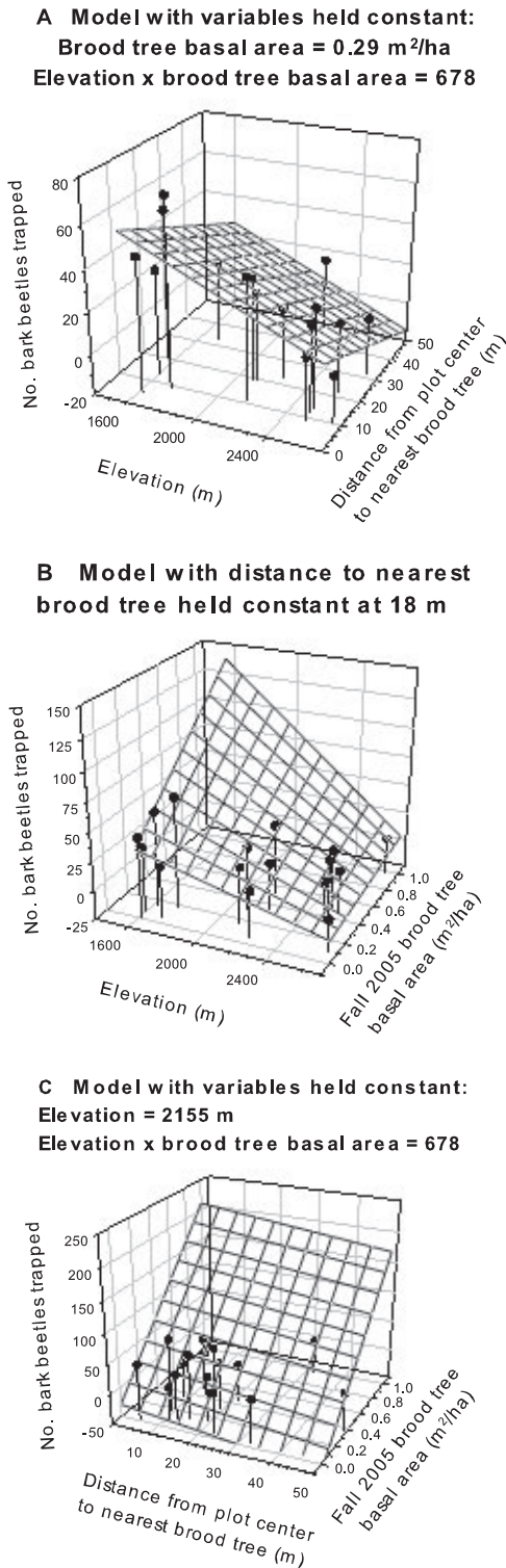
Fig. 3. Three-dimensional multiple regression response surfaces overlaid on the observed data points (solid circles with lines extending down to the bottom plane of the graph) for mean weekly trap catches of all bark beetles at 16 funnel trap sites in north-central Arizona in 2005 (see Table 4C for
