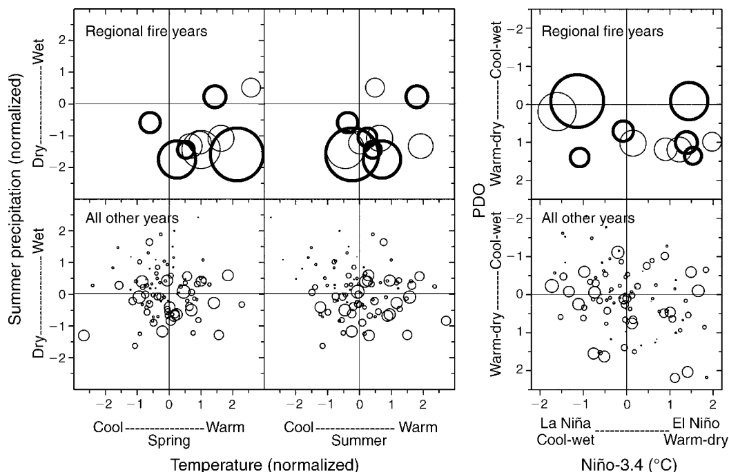
FIG. 5. Combined influence of spring (March–May) and summer (June–August) climate (left) and large-scale climate patterns (right) on regional-fire years (top) and all other years (1900–2003; bottom). Area of the circles is proportional to annual fire extent in the northern Rockies (minimum nonzero fire extent was 81 ha; maximum was 1 167 458 ha). Regional-fire years that occurred early in the 20th century (i.e., 1910–1934) are indicated with heavy circles. Precipitation and temperature are averages for the five climate divisions covered by the fire atlas, normalized over the analysis period (1900–2003). ENSO and PDO primarily affect spring climate in this region.
