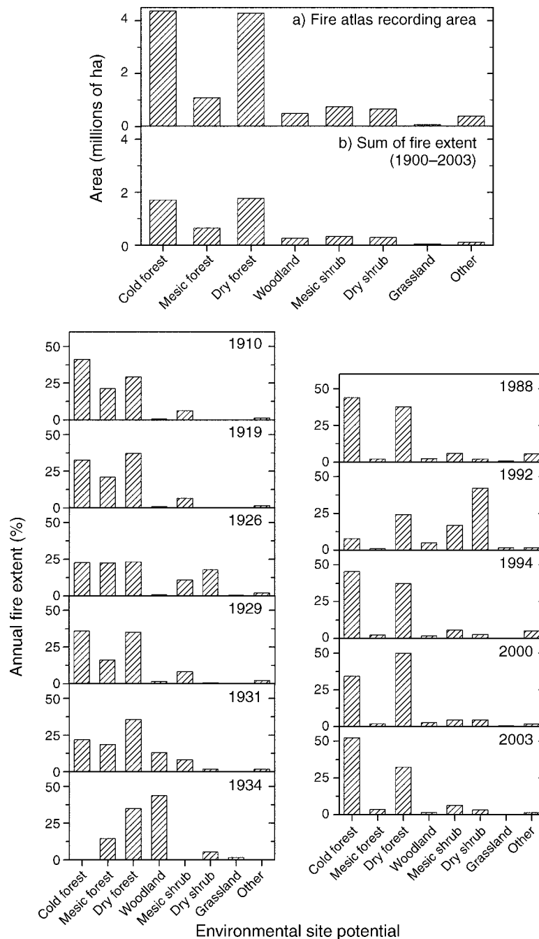
FIG. 6. The upper panel shows the area in each vegetation type (ESP, environmental site potential) (a) within the fire atlas recording area and (b) for total fire extent from 1900 to 2003 by vegetation type. Lower panels show the distribution of fire extent by potential vegetation during each of the 11 regional-fire years (from 1900 to 2003). Regional-fire years in the left column occurred early in the 20th century, while those in the right column occurred late in the 20th century. No regional-fire years occurred between 1935 and 1987.
