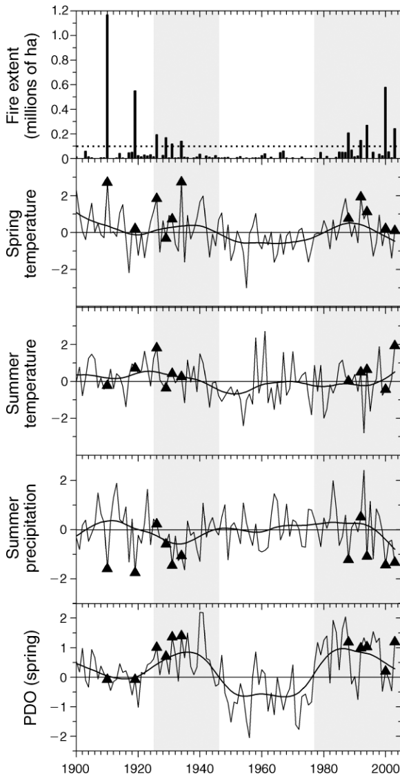
FIG. 3. Annual fire extent and 20th-century climate in the northern Rockies. The 11 years exceeding the 90th percentile in annual fire extent (102314 ha, horizontal dotted line) were identified as regional-fire years (top) and indicated with triangles in the other plots. Spring temperature (March–May), summer temperature (June–August), and summer precipitation were normalized then averaged over the five climate divisions covered by the fire atlas (1900–2003; see Methods: Climate drivers of regional-fire years for details). Heavy lines are climate data smoothed with cubic smoothing splines that retain 50% of the variance at periods of 25 years. Positive phases of the Pacific Decadal Oscillation (PDO) are shaded (Mantua et al. 1997).
