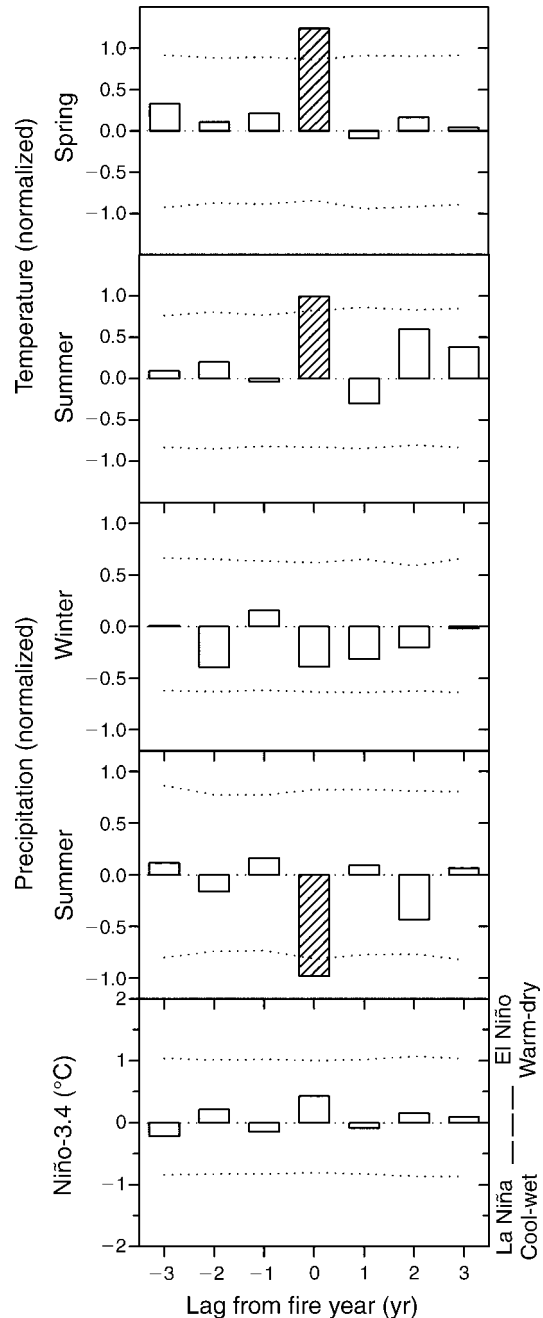
FIG. 4. Lagged annual relationship of fire and climate (spring [March–May] and summer [June–August] temperature, prior winter [December–February] and summer precipitation) or large-scale climate patterns (Niño-3.4 [December–February] as an index of ENSO), showing average departures during the 11 years exceeding the 90th percentile in annual fire extent across the northern Rockies from 1900 to 2003, and the years preceding and following such years. Hatched bars indicate departures that exceed 99% confidence intervals (dotted lines). Precipitation and temperature are averages for the five climate divisions covered by the fire atlas recording area, normalized over the analysis period (1900–2003).
