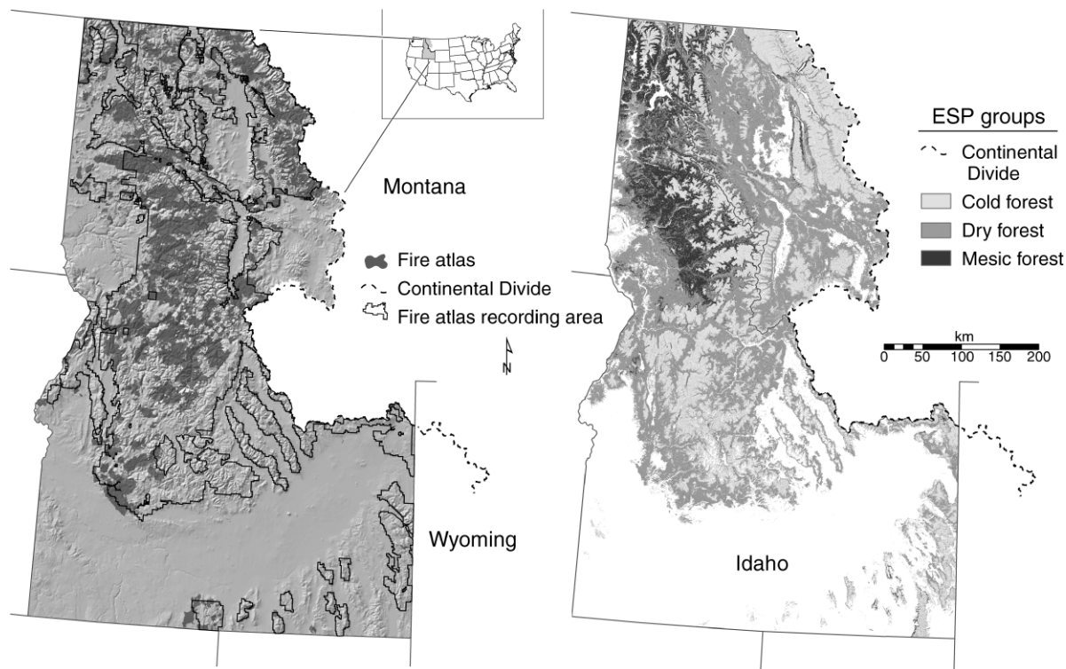
FIG. 1. The U.S. northern Rockies study area in Idaho and Montana west of the Continental Divide. Our 120 708-ha fire atlas recording area (left) is reported from 12 national forests and one national park. Burned polygons (1900–2003) are shown in dark gray against a background of elevation. The three most extensive types of potential vegetation (identified by environmental site potential [ESP], right) cover 81% of the fire atlas recording area. A small amount of the total fire extent (657 983 ha, 5% of the fire atlas recording area) lies outside the boundaries of the fire atlas recording area.
