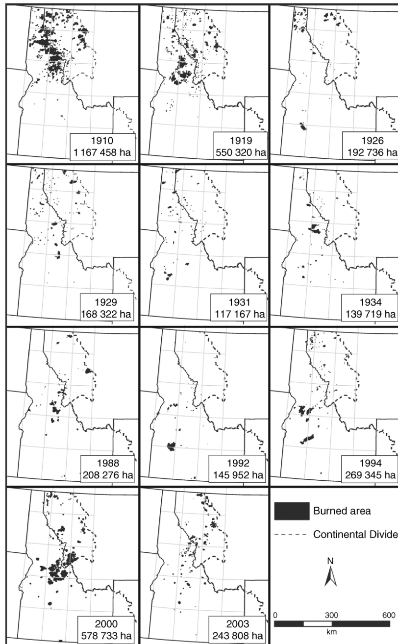
FIG. 2. Fires were widespread during each of the eleven 20th-century regional-fire years identified for the northern Rockies. The grid cells are 1.5^\circ latitude by 1.5^\circ longitude, and all 17 grid cells shown had burned polygons in them in at least one year, though not necessarily in one of the regional-fire years shown here.
