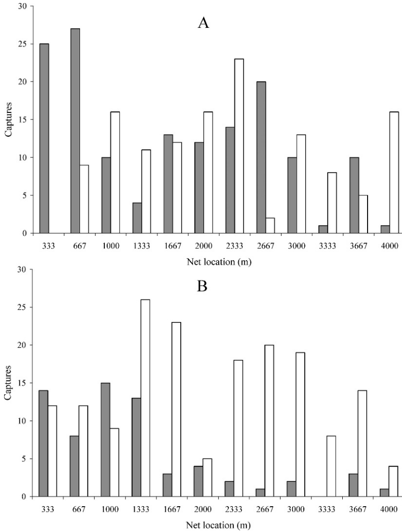
FIG. 2. Hoop-net captures of juvenile (gray bars) and adult (white bars) Boreal Toads by net location date in Little Blue Joint Creek (A) and Slate Creek (B) in summer 2003.
