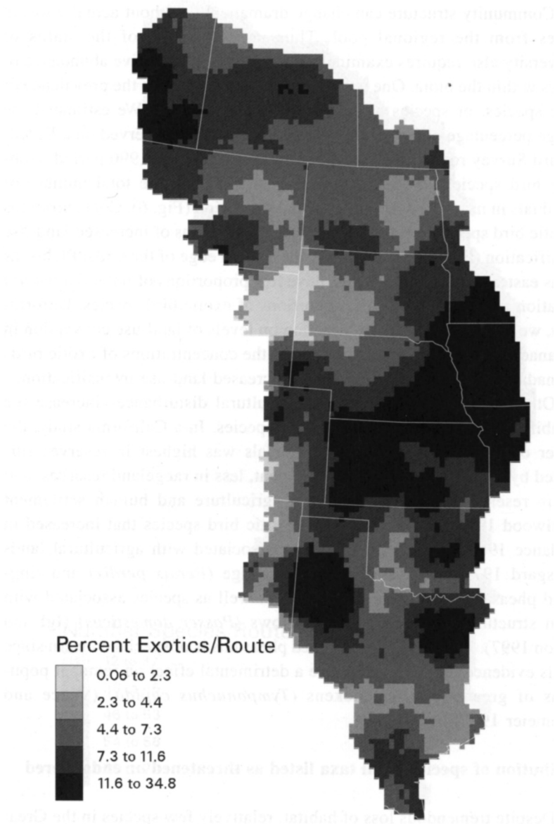
Figure 6. Average percentage of breeding birds that are exotic species. Plots were generated by kriging (Cressie 1991) percentage of exotic species across all Breeding Bird Survey routes in the Great Plains.
