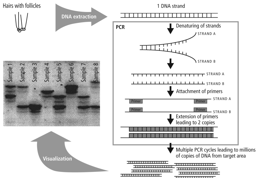
Figure 9.1. Schematic illustrating the process of deriving individual identification from hair samples. This process begins with DNA extraction, which produces DNA strands. Next, a particular region of the DNA is amplified using (in this case) microsatellite primers, and the polymerase chain reaction (PCR). The PCR process involves three major steps: (1) the denaturing of the double-stranded DNA molecule; (2) the attachment of primers at a particular locus in the genome; and (3) the extension of these primers to produce a copy of the original locus. After multiple PCR cycles, millions—if not billions—of copies of the region are created, and can then be visualized on an electrophoresis gel. This gel image shows eight Canada lynx samples evaluated at one microsatellite locus. Even with one locus, multiple individuals can already be discerned, but samples 5 and 7 produce the same banding pattern at this locus. Ultimately, when additional loci were run, these two samples were determined to be from different individuals.
