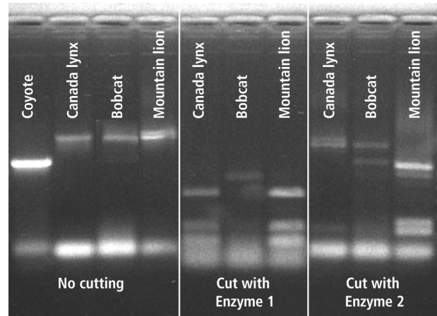
Figure 9.2. An electrophoresis gel showing the results of a restriction digest test to determine species identification. Without deploying any restriction enzymes, separation of felids and canids is possible. Using two different enzymes, Canada lynx, bobcats, and mountain lions can be discerned.
