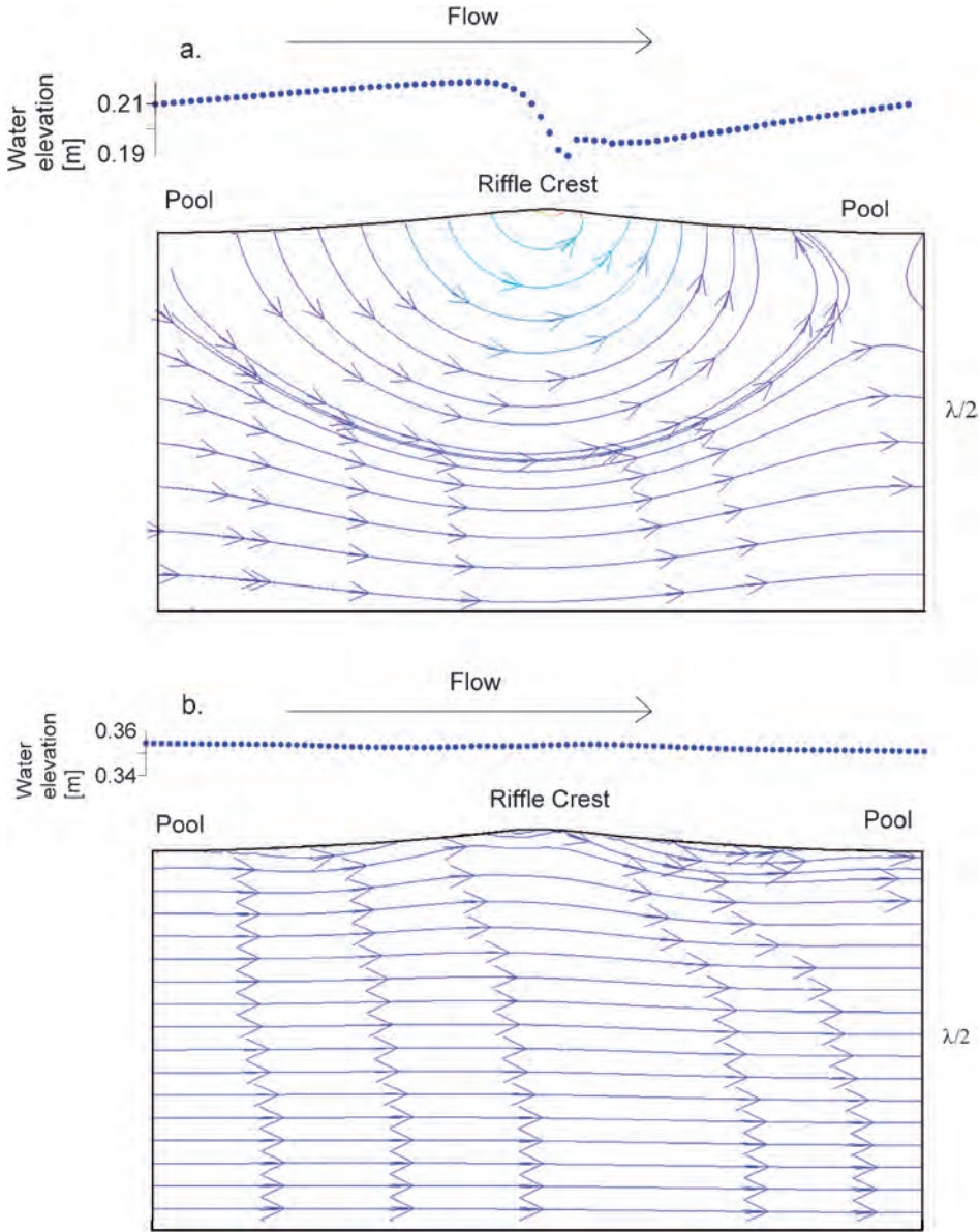
Figure 5.7. Simulated hyporheic pathlines for a synthetic two-dimensional pool-riffle topography with (a) low discharge (8% bankfull flow) and (b) high discharge (100% bankfull flow). Channel characteristics scaled from natural gravel-bed rivers in central Idaho: slope is 0.5% and the ratio of bedform amplitude to wavelength, \Delta/\lambda , is 0.03. Surface and subsurface flow simulated using MD_SWMS 1 (McDonald et al., 2005) and FLUENT 6.0 (FLUENT Inc.), respectively. Predicted water surface profiles are plotted separately above each panel at exaggerated vertical scales to emphasize their differences, but do not indicate flow depths over bed topography. Subsurface flow simulations use a uniform hydraulic conductivity of 0.1 \text{ cm s}^{-1} (sandy gravel), with lighter-coloured hyporheic pathlines indicating faster flow.
