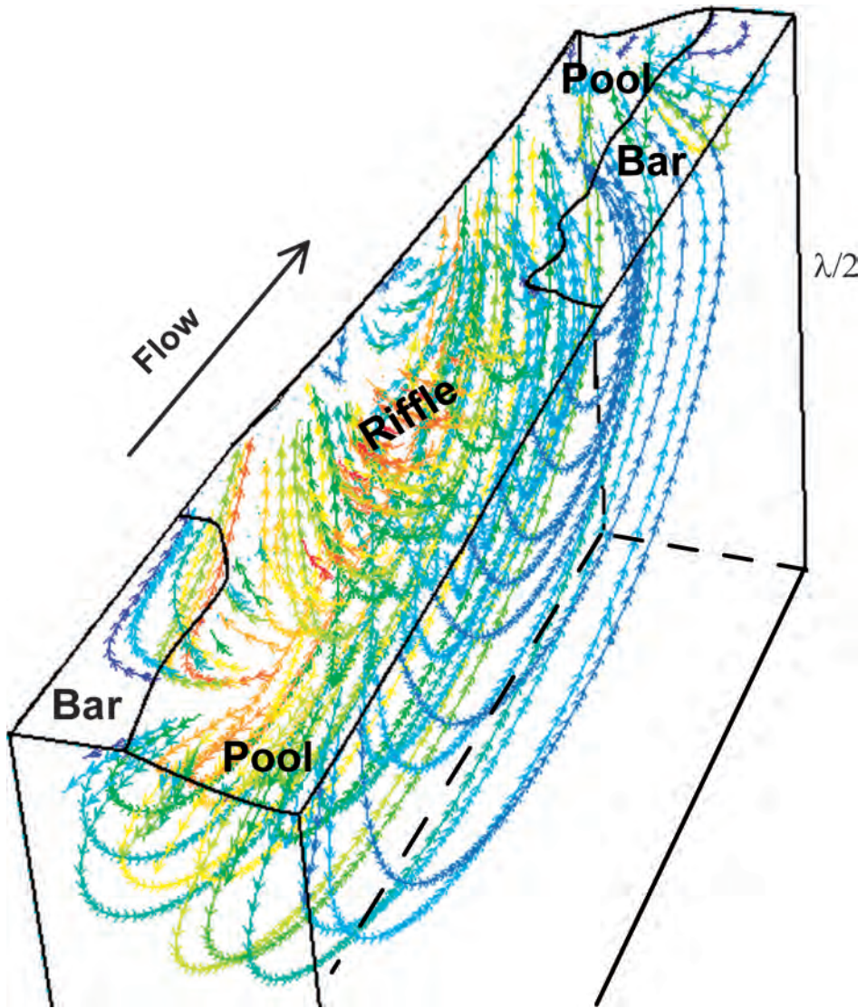
Figure 5.8. Simulated hyporheic pathlines for a synthetic three-dimensional pool-riffle channel with alternate bar morphology and low discharge (26% bankfull flow). Channel characteristics scaled from natural gravel-bed rivers in central Idaho: slope is 0.41% and the ratio of bedform amplitude to wavelength is 0.022 (Tonina and Buffington, 2007, experiment 1). Surface and subsurface flow simulated using FLUENT 6.0 (FLUENT Inc.), with hyporheic pathlines originating from the surface and coloured by individual trajectory. The simulation uses a groundwater slope of 0.41%, a uniform hydraulic conductivity of 5 \text{ cm s}^{-1} (Tonina and Buffington, 2007), and an alluvial depth equal to one bedform wavelength ( 1\lambda ). Deeper groundwater flow paths (those that do not intersect the bed surface) are not shown.
