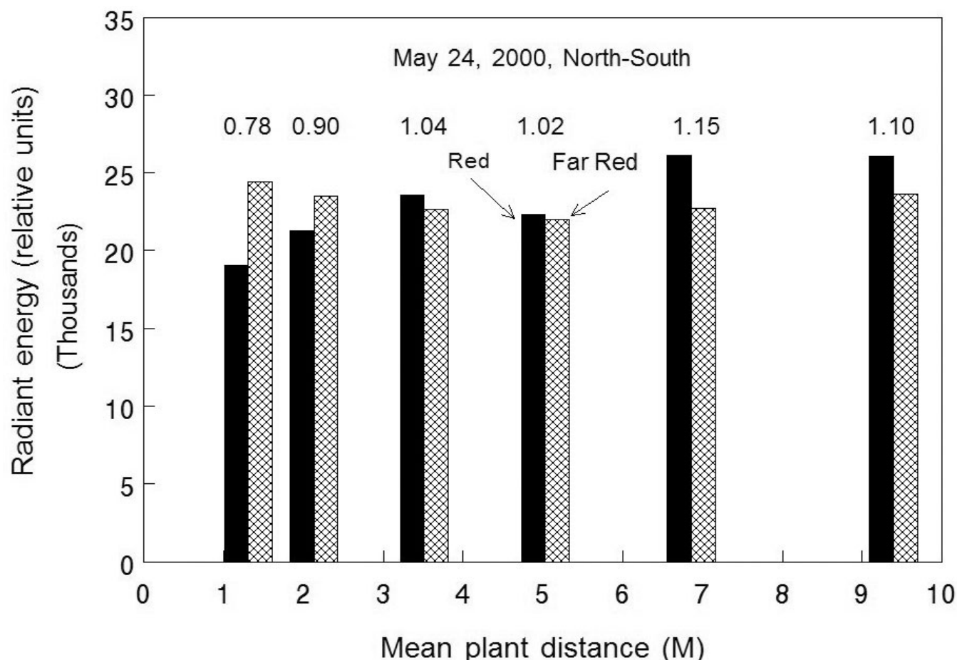
Figure 6 —Red and far red light intensity measured at varying mean plant distances in a Nelder plot. Numbers above bars are R/FR.
