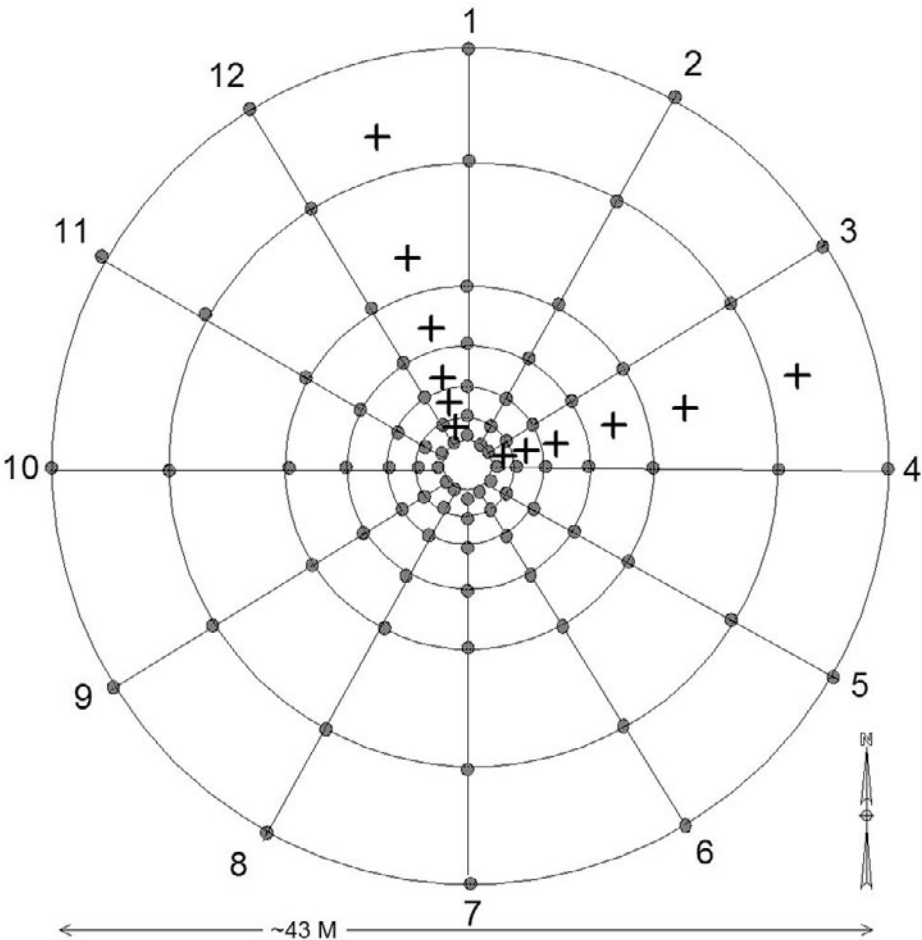
Figure 1 —Diagram of the Nelder (1962) plot established to test the effect of planting density on R/FR light and tree growth. Each point indicates the location of one Douglas-fir plant. Each + is a light measurement point. “Spokes” are numbered 1 to 12.
