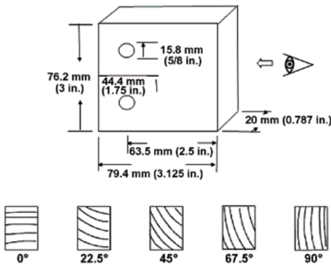
Figure 5—Test specimens for mode I fracture testing. Orientation recorded is shown by degrees.
