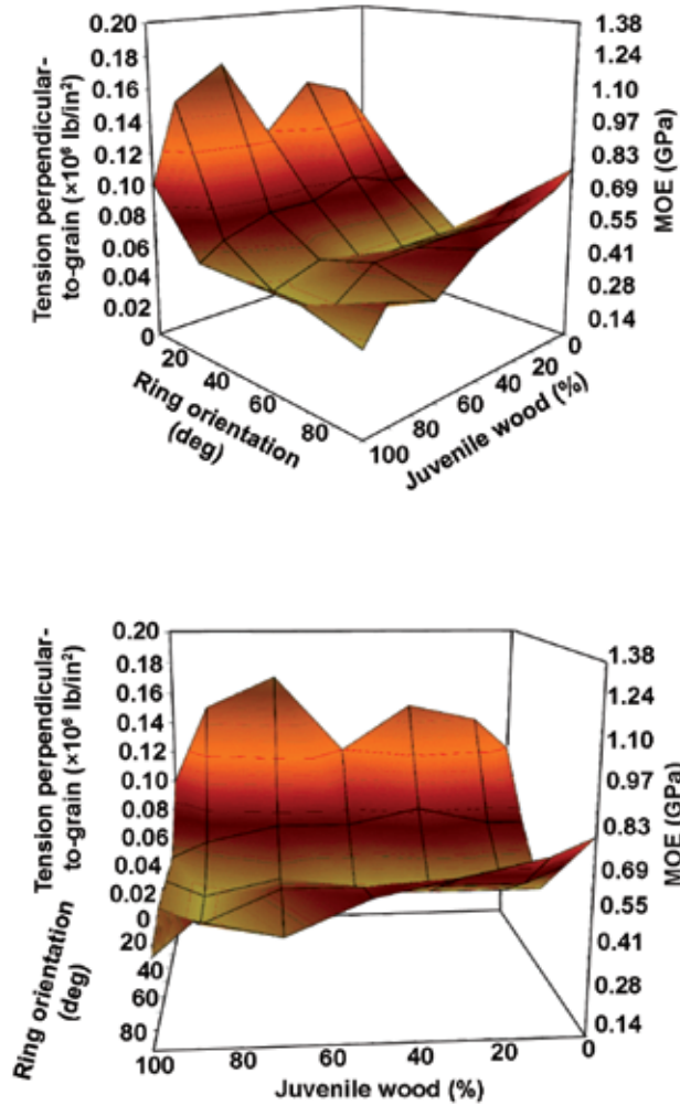
Figure 14—The effect of juvenile wood on modulus of elasticity (MOE) for tension perpendicular-to-grain at various orientations.
