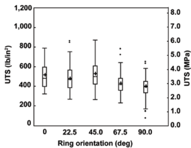
Figure A11—Ultimate tensile stress (UTS) perpendicular-to-grain for ASTM specimen compared with growth-ring orientation.
