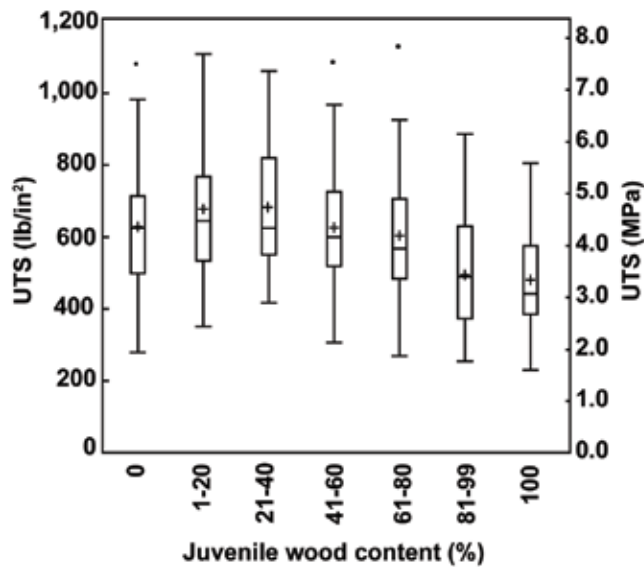
Figure A5—Dog-bone specimen ultimate tensile stress (UTS) perpendicular-to-grain compared with juvenile wood content.
