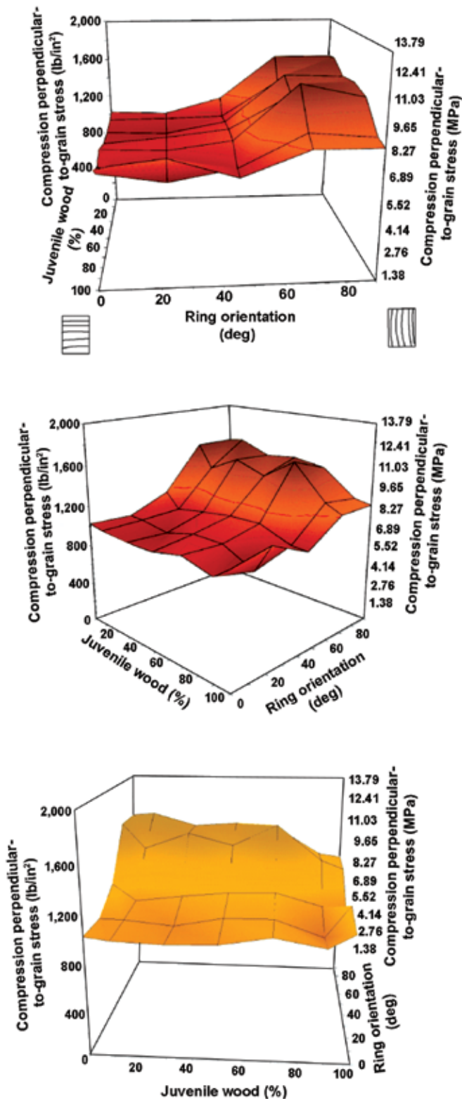
Figure 8—The effect of juvenile wood on compressive stress perpendicular-to-grain at 1-mm (0.04-in.) displacement for various orientations.
