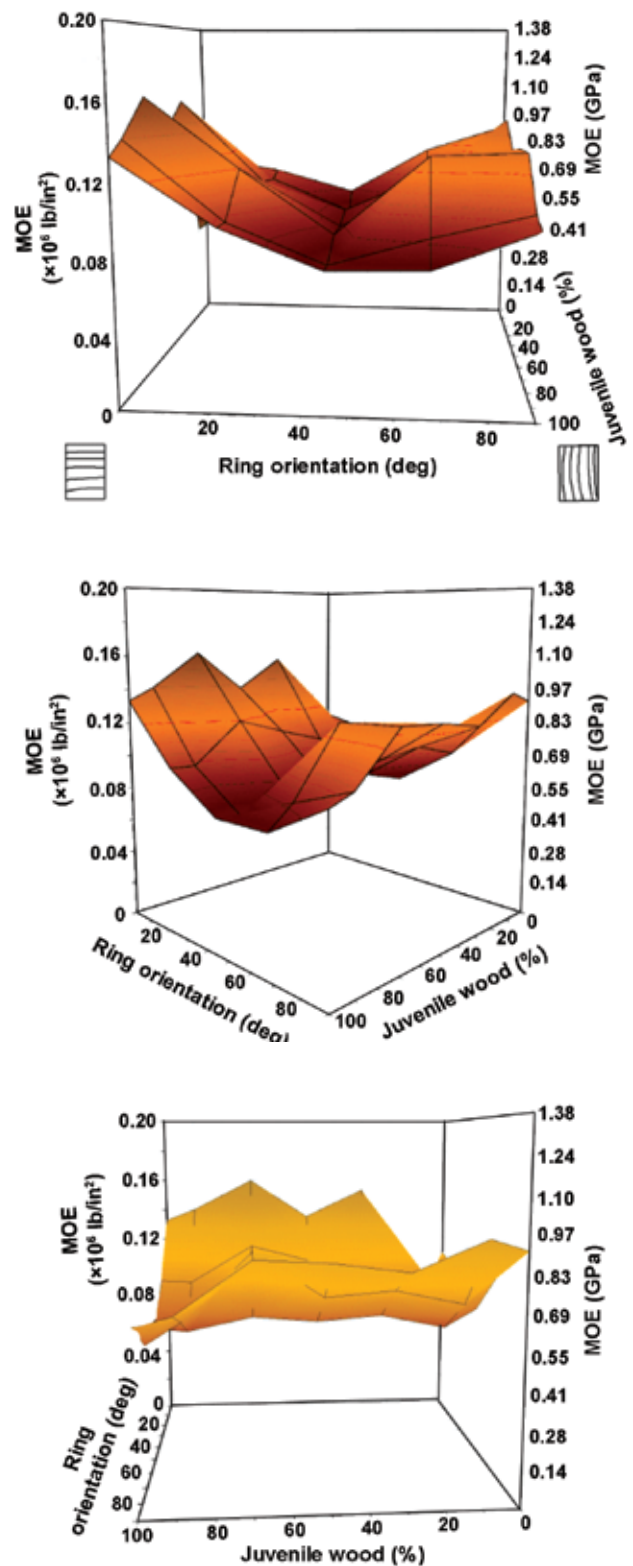
Figure 9—The effect of juvenile wood on modulus of elasticity (MOE) perpendicular-to-grain for various orientations.
