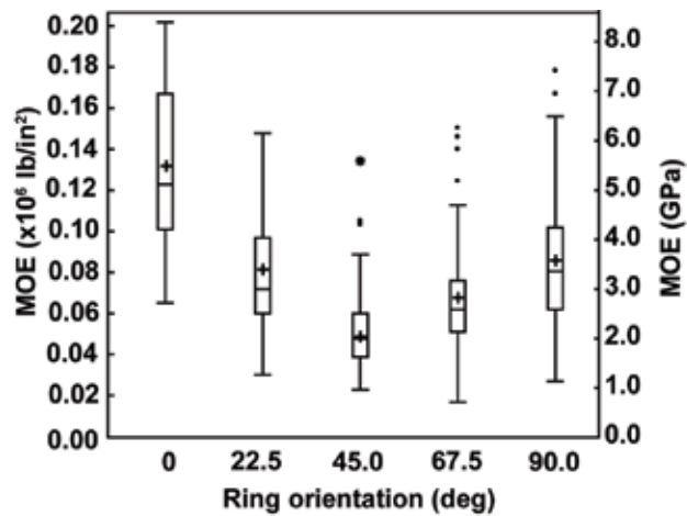
Figure A13—Modulus of elasticity (MOE) for tension perpendicular-to-grain dog-bone specimen compared with growth-ring orientation.
