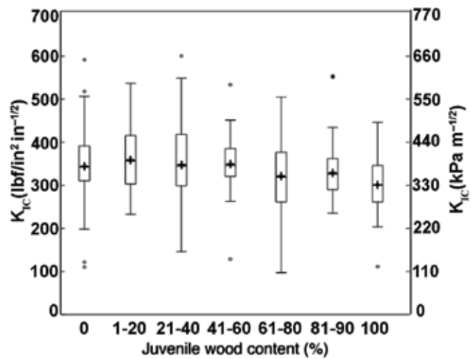
Figure A7—Mode I fracture toughness compared with juvenile wood content.
