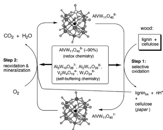
Fig. 3. Thermodynamically stable, self-buffering system for selective use with \text{O}_2 as the oxidant in \text{H}_2\text{O} as the solvent, illustrated in this case by the delignification of wood. Step 1 involves selective oxidation of the lignin in wood or wood pulp by the oxidizing POM, [\text{AlV}^{\text{V}}\text{W}_{11}\text{O}_{40}]^{6-} . The protons that are generated by oxidations in water are consumed by the more basic POMs present in the equilibrating POM ensemble, [\text{Al}_3\text{W}_{10}\text{O}_{38}]^{7-} , [\text{Al}_2\text{W}_{11}\text{O}_{39}]^{6-} , [\text{V}_2\text{W}_4\text{O}_{19}]^{4-} and [\text{W}_7\text{O}_{24}]^{6-} . The oxidized lignin fragments are soluble and easily removed from the cellulose, which can be further processed to generate paper products. Step 2 involves reoxidation of the reduced POM, [\text{AlV}^{\text{IV}}\text{W}_{11}\text{O}_{40}]^{7-} , while the hydroxide generated by coupled \text{O}_2 reduction is again consumed by the equilibrating POM ensemble. The equilibrating ensemble consumes, alternatively, both \text{H}^{+} and \text{OH}^{-} keeping the pH approximately neutral as the cycle is repeated many times.
