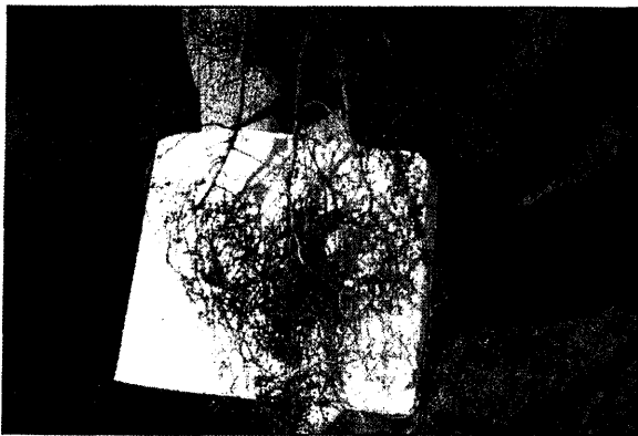
Figure 11. October root systems of 2+0 Scots pine seedlings pruned to 10 cm at the beginning of the second growing season at the Zhanggutai Nursery.
