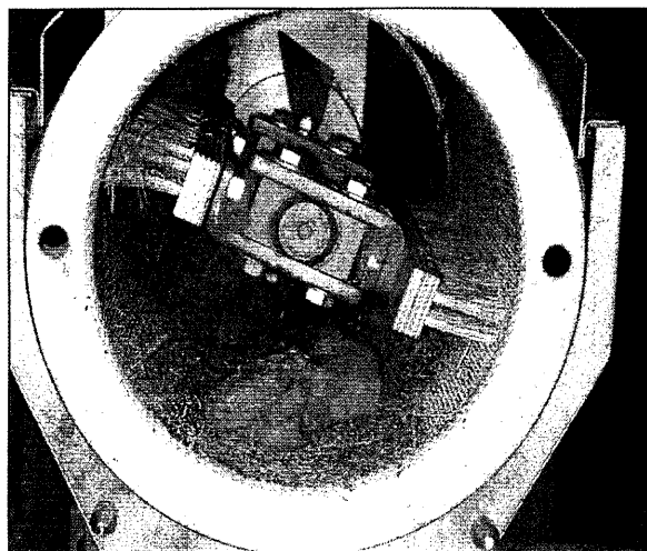
Figure 4. Brushes and mantle in use.
