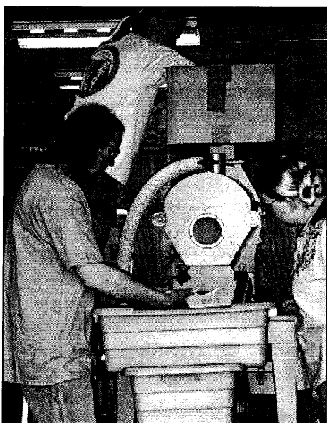
Figure 2. Operation of the Westrup brush machine.
