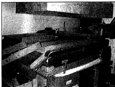
Figure 5. Specific gravity table for conditioning seeds.
