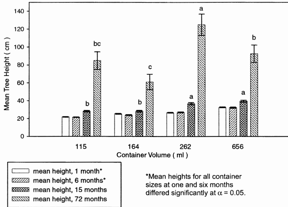
Figure 4. Mean height by stock size for Arizona cypress planted in fall 1994 at Los Lunas. Means within same letter groupings did not differ significantly within each year at \alpha = 0.05 .
