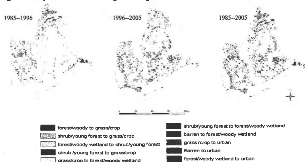
Figure 5. Major Land Cover Changes During 20 Years
