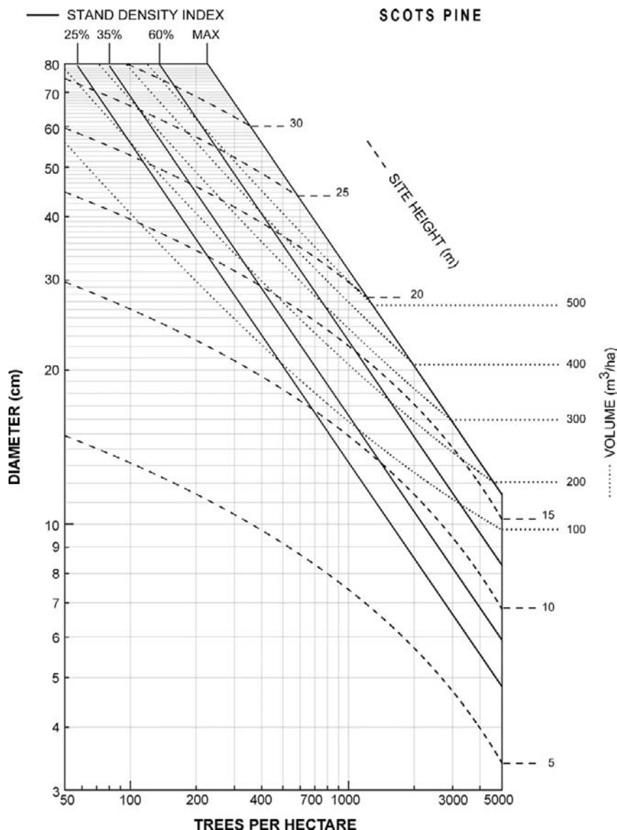
Fig. 5. Density management diagram for Scots pine in the western Italian Alps.
