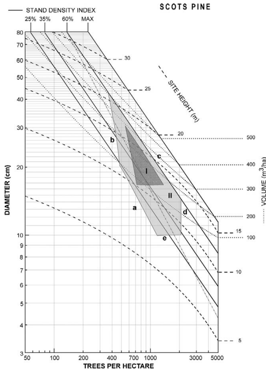
Fig. 6. Suitability zone for optimal (I) and minimal (II) protection from rockfall. Size-density combinations determining complete canopy closure (dash and dotted line) are superimposed on the DMD. Suitability zones are defined by (a) minimum crown closure; (b) minimum MTFD; (c) minimum crown ratio; (d) maximum tree slenderness; (e) minimum QMD.
