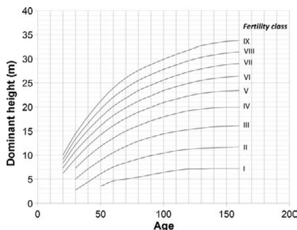
Fig. 7. Site index curves for Scots pine used in this study (adapted from Wiedemann, 1949). Model form and measures of statistical significance were not specified by the source.
