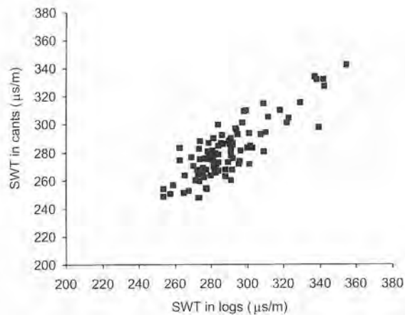
Figure 3.1. — Relationship of stress wave transmission time (SWT) in logs and SWT in cants.
