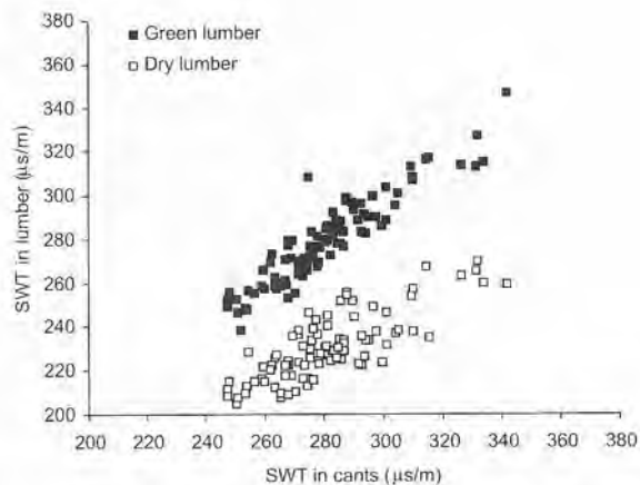
Figure 3.3. — Relationship of stress wave transmission time (SWT) in cants and SWT in lumber.
