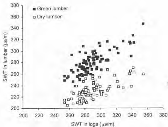
Figure 3.2. — Relationship of stress wave transmission time (SWT) in logs and SWT in lumber.
