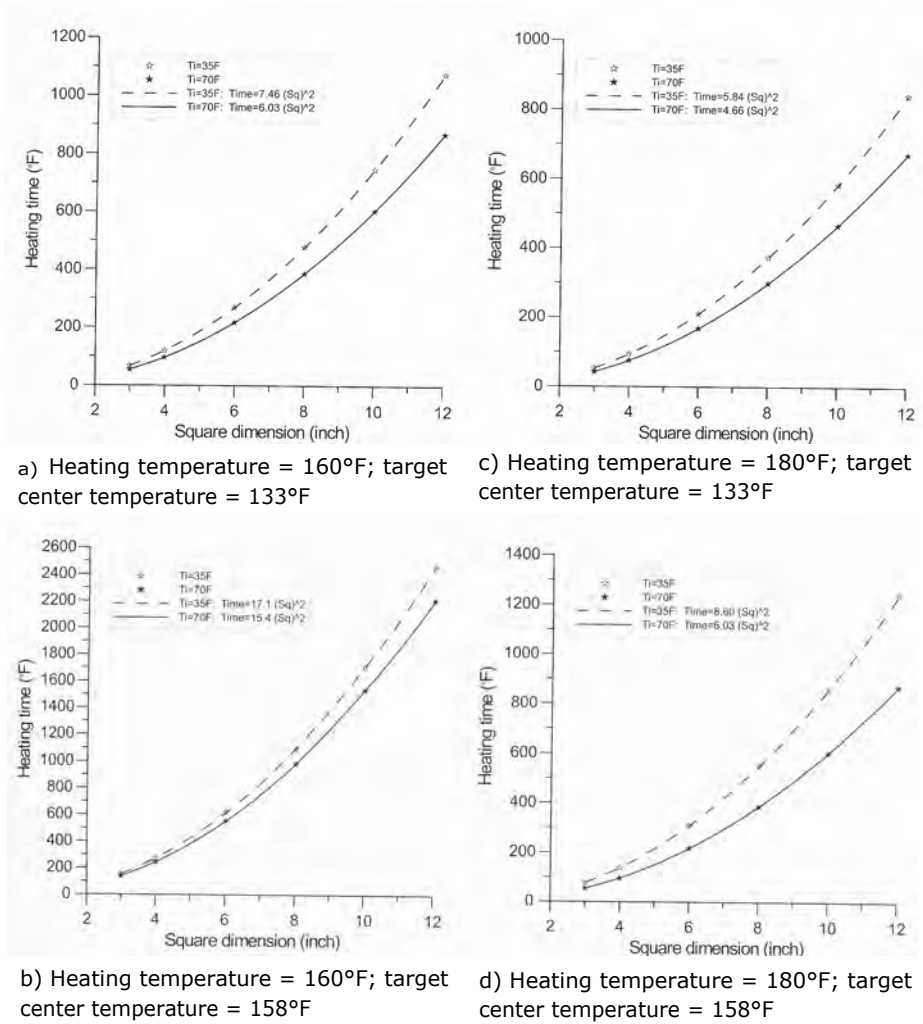
Figure 5.5. — Graphs of the time required to heat the center of square maple timbers to a target temperature versus the dimension of the square timber.
