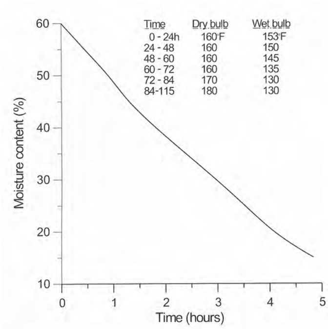
Figure 5.3. — Graph of moisture content versus time for 2- by 6-inch maple lumber kiln-dried by a time-based schedule.
