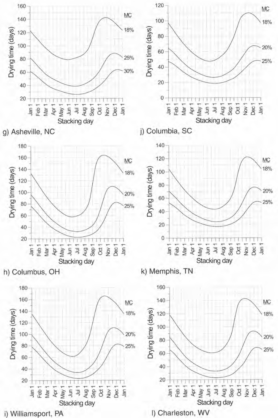
Figure 5.1 (continued). — Estimated air-drying times for nominal 2- by 6-inch maple lumber as they depend on geographical location, stacking date, and final moisture content.
