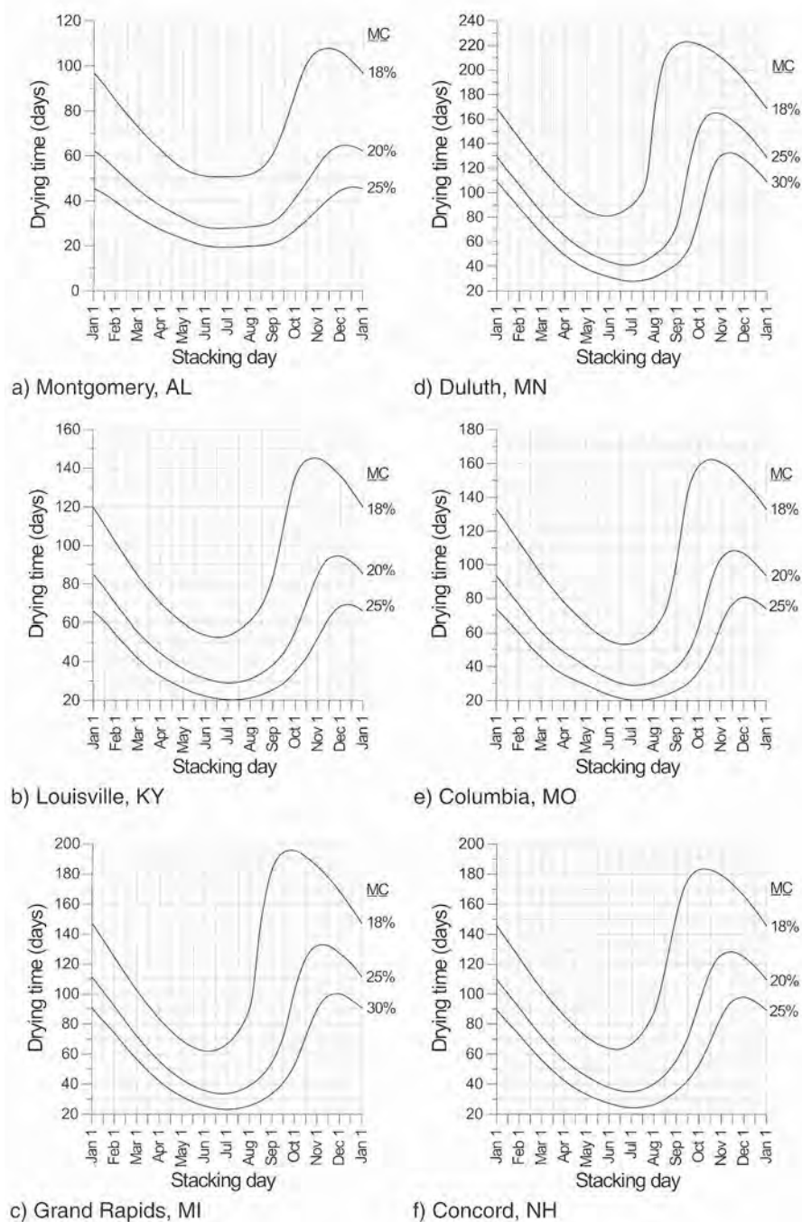
Figure 5.1. — Estimated air-drying times for nominal 2- by 6-inch maple lumber as they depend on geographical location, stacking date, and final moisture content. ( Figure continued on next page. )
