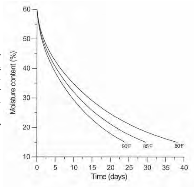
Figure 5.2. — Graphs of moisture content versus time for 2- by 6-inch maple lumber in a pre-dryer at three temperature levels (80°, 85°, and 90°F) and 65 percent relative humidity.
