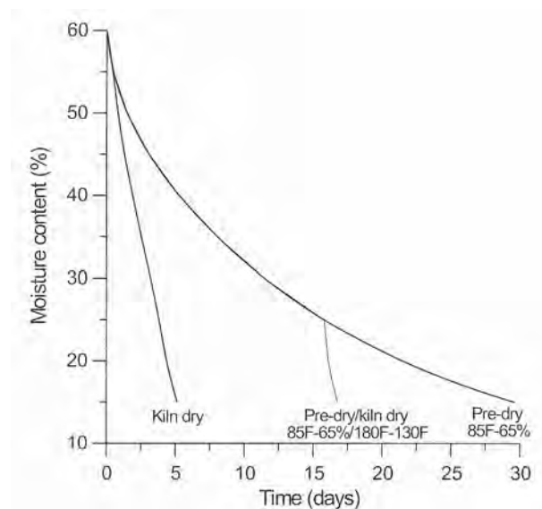
Figure 5.4. — Graph of moisture content versus time for 2- by 6-inch maple lumber dried in a kiln, in a pre-dryer, and sequentially in a pre-dryer and then a dry kiln.
